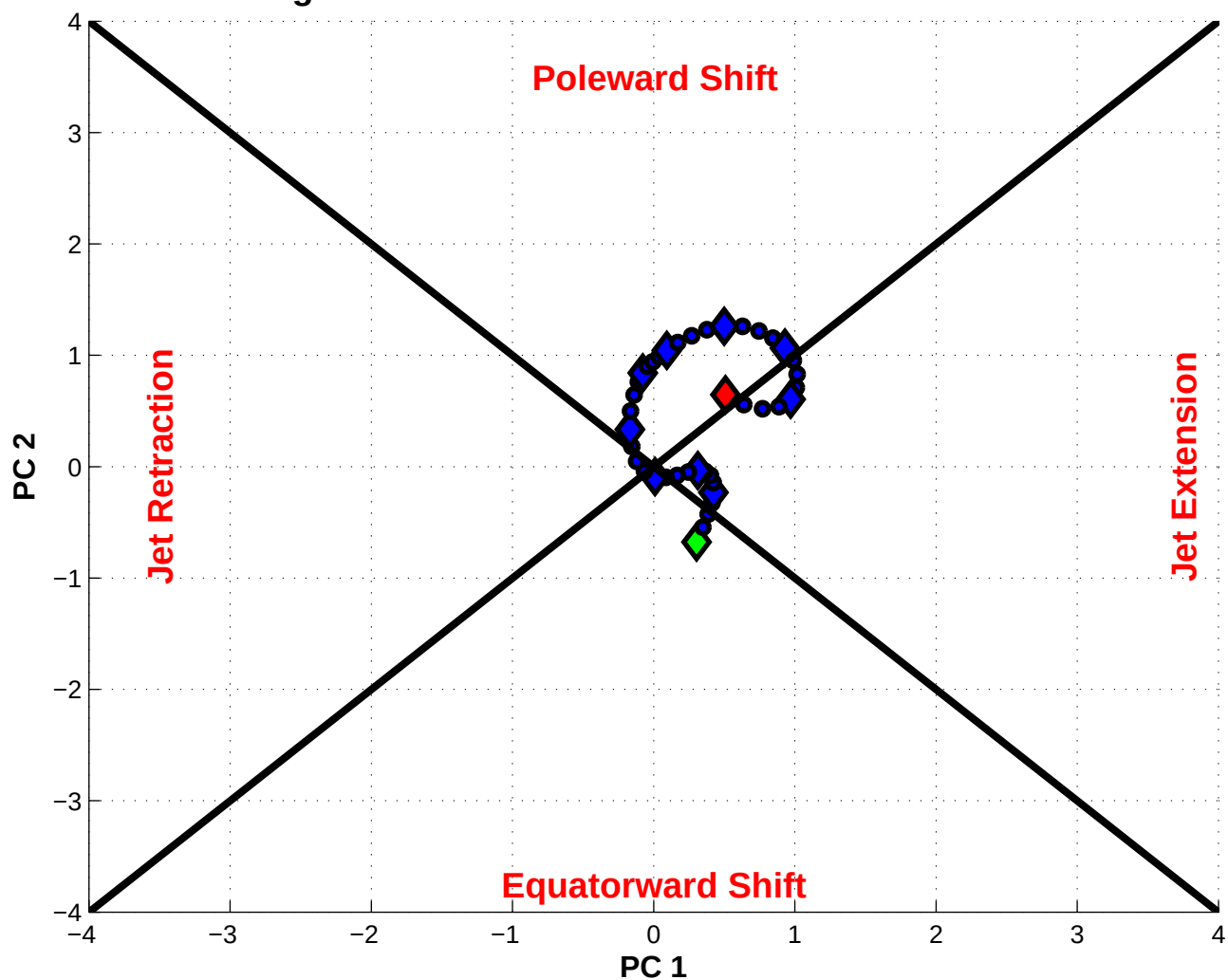
NPJ Phase Diagram valid 1200 UTC 19 Feb 1993 – 1200 UTC 01 Mar 1993
