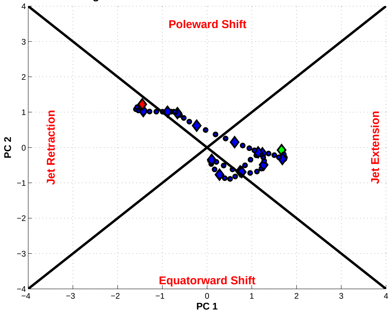
NPJ Phase Diagram valid 0000 UTC 20 Dec 1985 – 0000 UTC 03 Jan 1986
