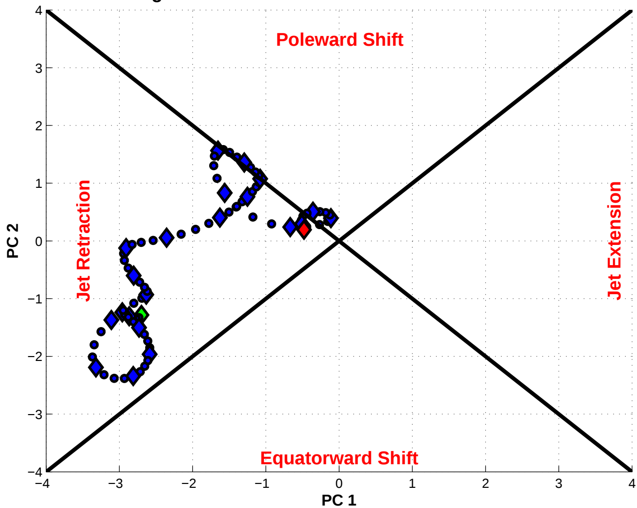
NPJ Phase Diagram valid 1800 UTC 20 Feb 2006 – 1200 UTC 14 Mar 2006
