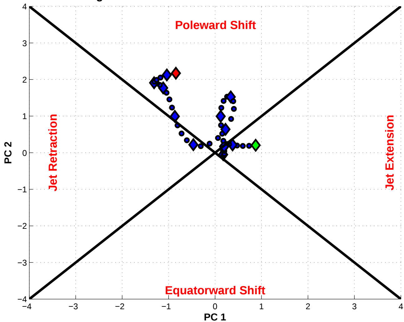
NPJ Phase Diagram valid 0000 UTC 22 Feb 2004 – 0600 UTC 05 Mar 2004
