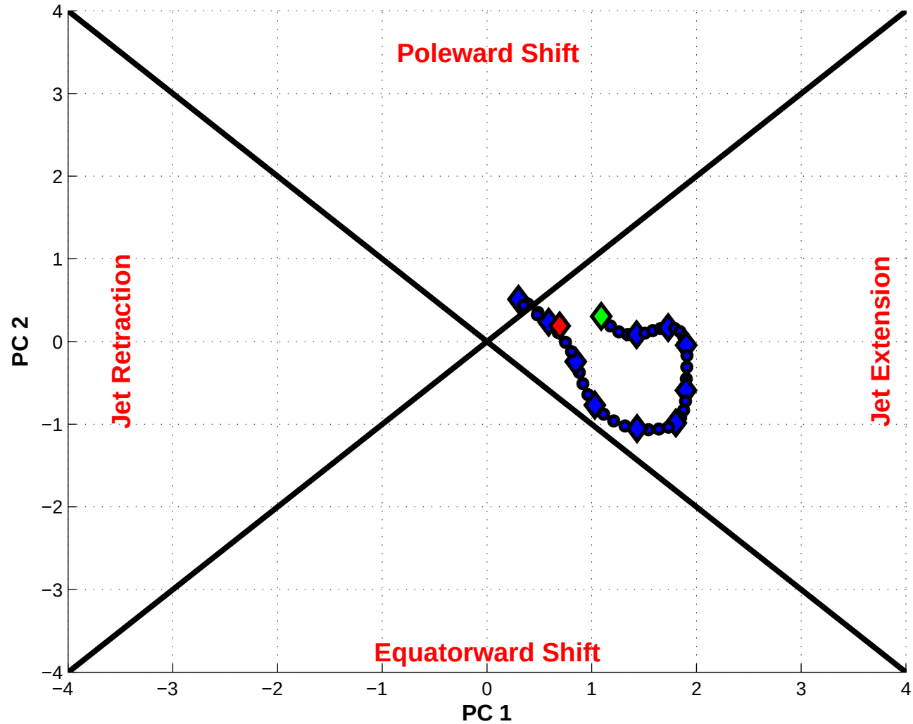
NPJ Phase Diagram valid 1200 UTC 25 Jan 1986 – 0600 UTC 05 Feb 1986
