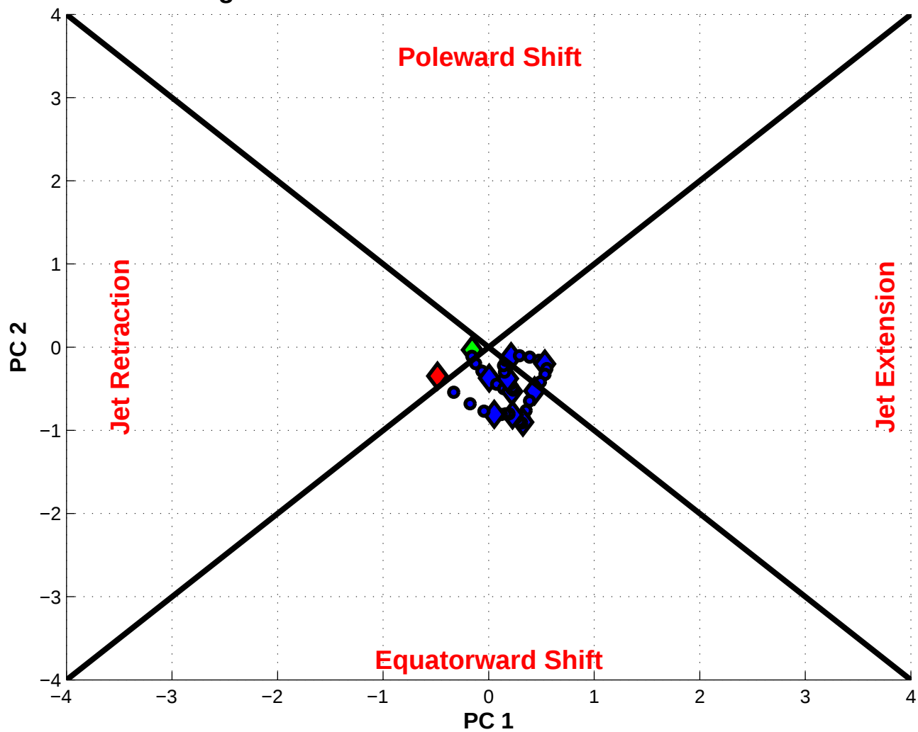
NPJ Phase Diagram valid 0600 UTC 29 Dec 1998 – 0600 UTC 08 Jan 1999
