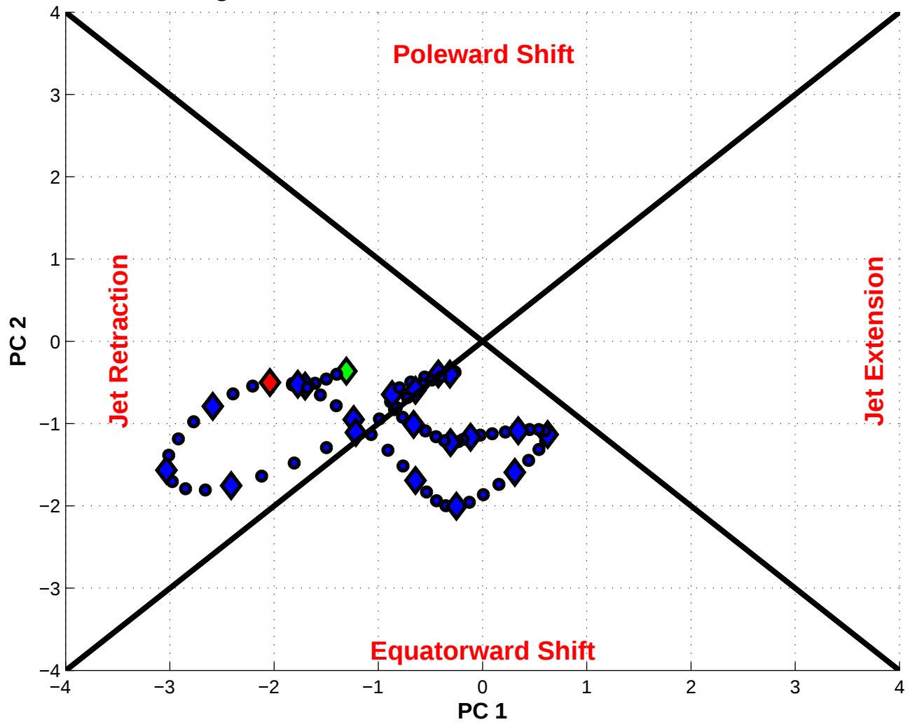
NPJ Phase Diagram valid 1200 UTC 02 Dec 2010 – 0600 UTC 22 Dec 2010
