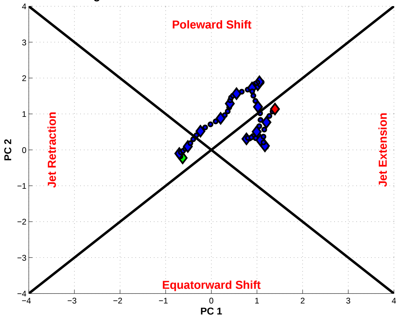
NPJ Phase Diagram valid 0600 UTC 03 Nov 1981 – 0000 UTC 19 Nov 1981
