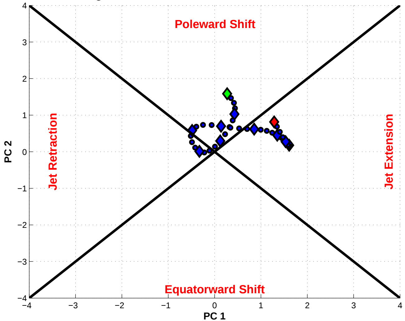
NPJ Phase Diagram valid 1800 UTC 04 Dec 1981 – 1800 UTC 14 Dec 1981
