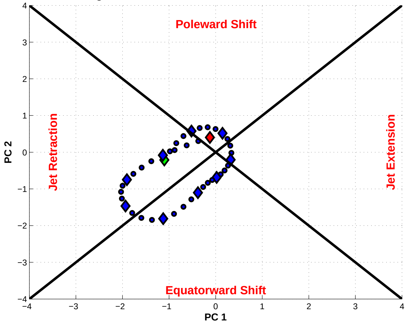
NPJ Phase Diagram valid 0600 UTC 04 Dec 1997 – 0600 UTC 14 Dec 1997
