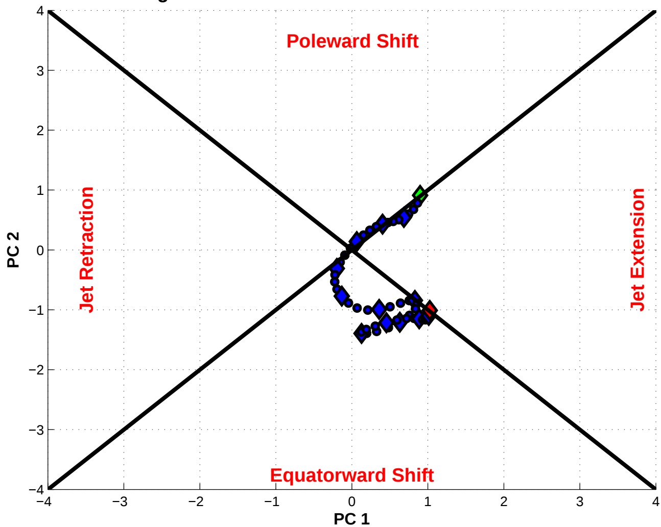
NPJ Phase Diagram valid 1800 UTC 04 Mar 1993 – 0000 UTC 17 Mar 1993
