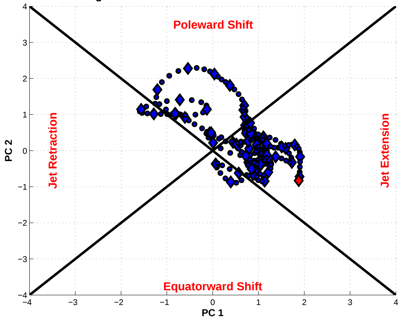
NPJ Phase Diagram valid 1800 UTC 05 Dec 1985 – 0000 UTC 30 Jan 1986
