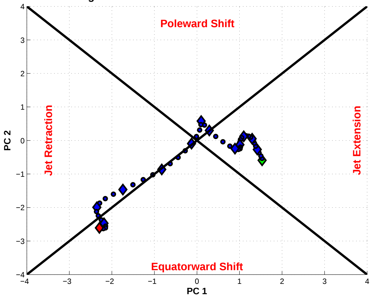
NPJ Phase Diagram valid 0000 UTC 05 Feb 1996 – 0000 UTC 18 Feb 1996
