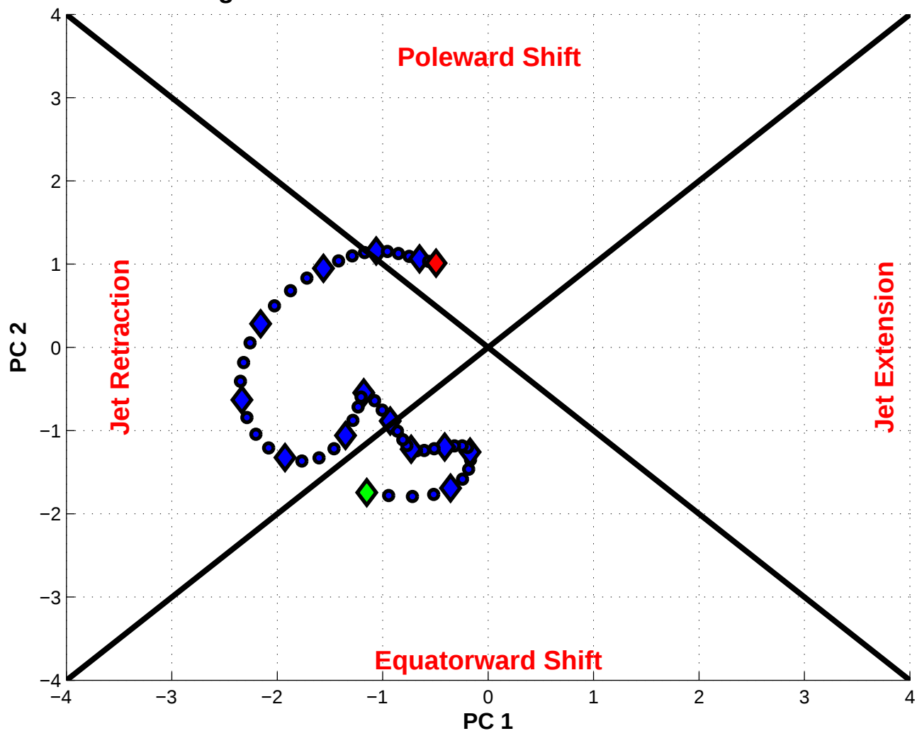
NPJ Phase Diagram valid 0000 UTC 05 Feb 2014 – 1200 UTC 18 Feb 2014
