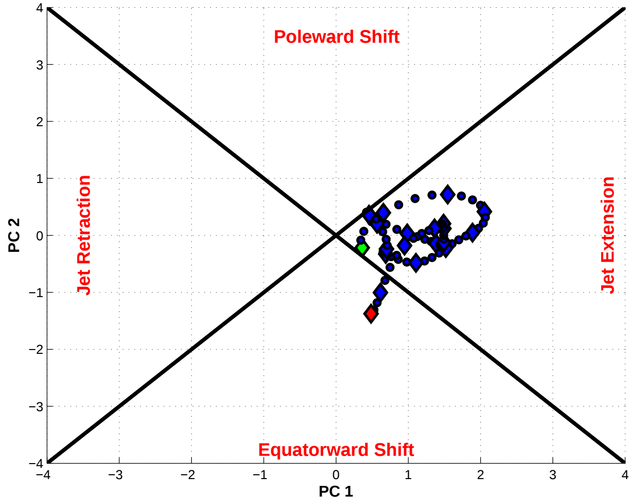
NPJ Phase Diagram valid 0000 UTC 05 Jan 1985 – 1800 UTC 23 Jan 1985
