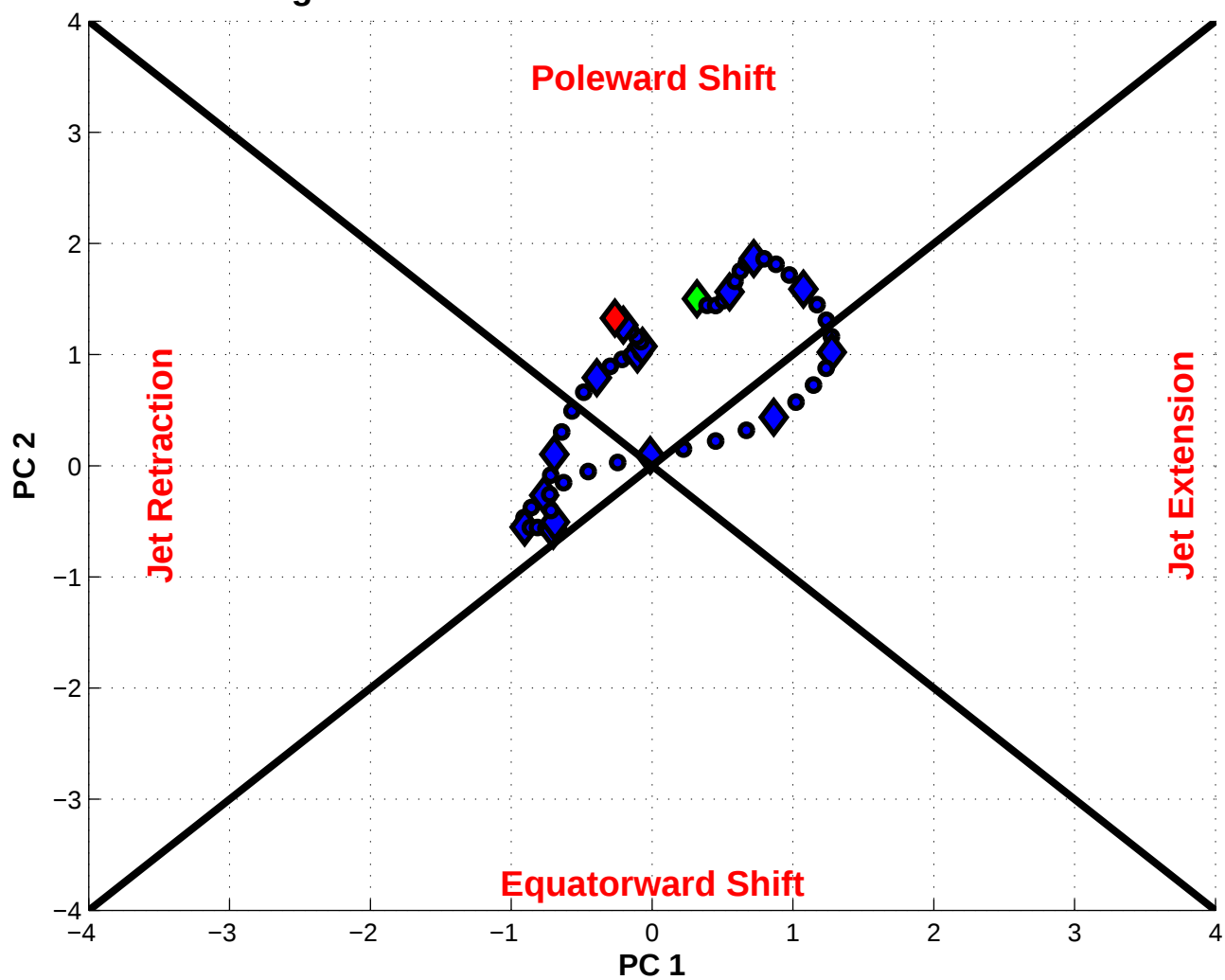
NPJ Phase Diagram valid 0600 UTC 06 Mar 1988 – 1200 UTC 21 Mar 1988
