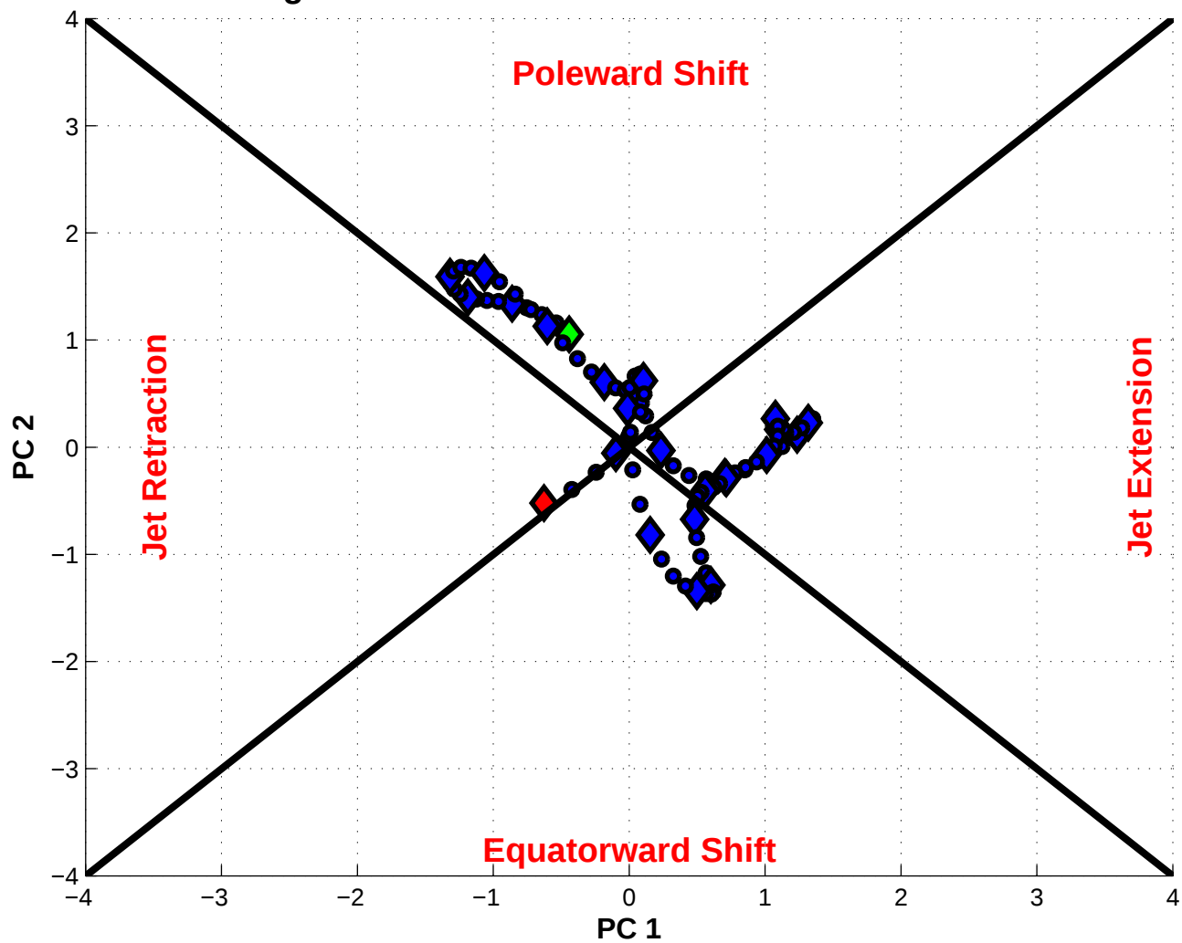
NPJ Phase Diagram valid 1200 UTC 07 Jan 2014 – 0600 UTC 31 Jan 2014
