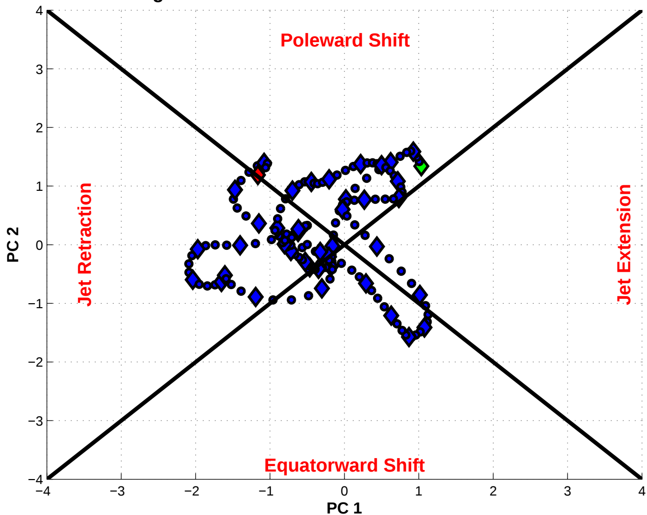
NPJ Phase Diagram valid 1200 UTC 10 Nov 2008 – 0600 UTC 21 Dec 2008
