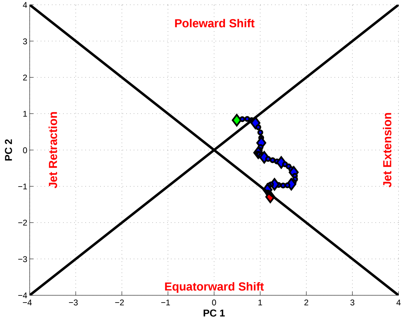
NPJ Phase Diagram valid 0600 UTC 11 Jan 1983 – 0000 UTC 21 Jan 1983
