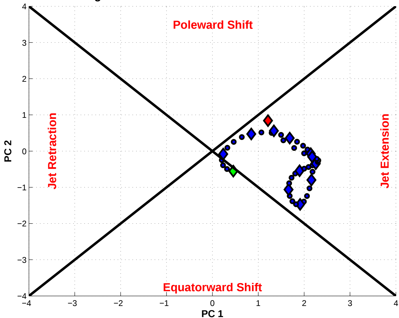
NPJ Phase Diagram valid 0000 UTC 12 Dec 2005 – 0600 UTC 23 Dec 2005
