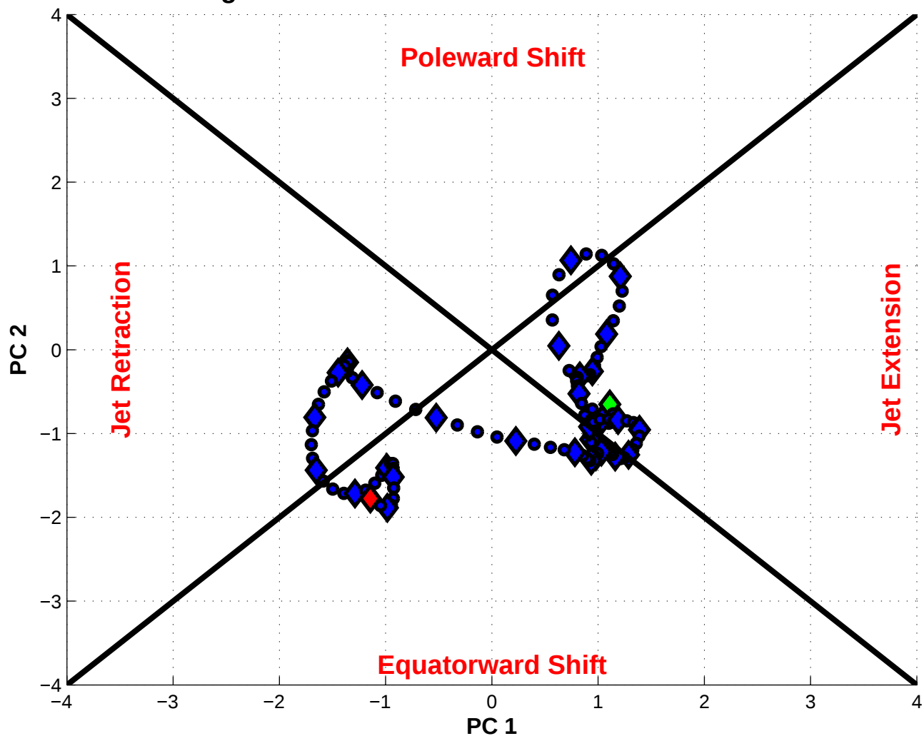
NPJ Phase Diagram valid 1800 UTC 12 Jan 1992 – 0600 UTC 11 Feb 1992
