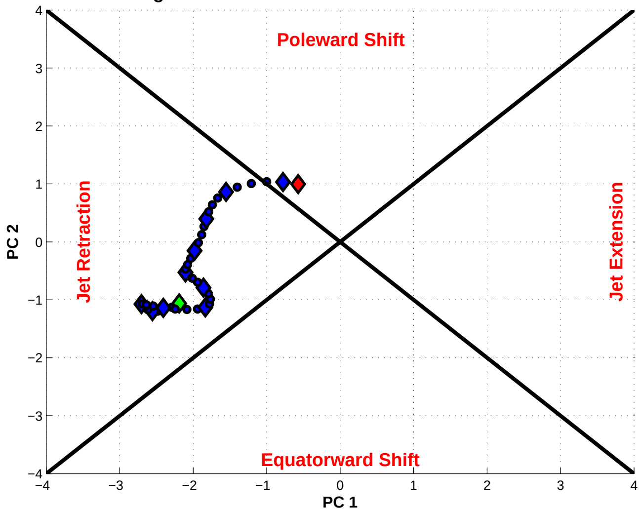
NPJ Phase Diagram valid 1200 UTC 13 Jan 2000 – 1800 UTC 23 Jan 2000
