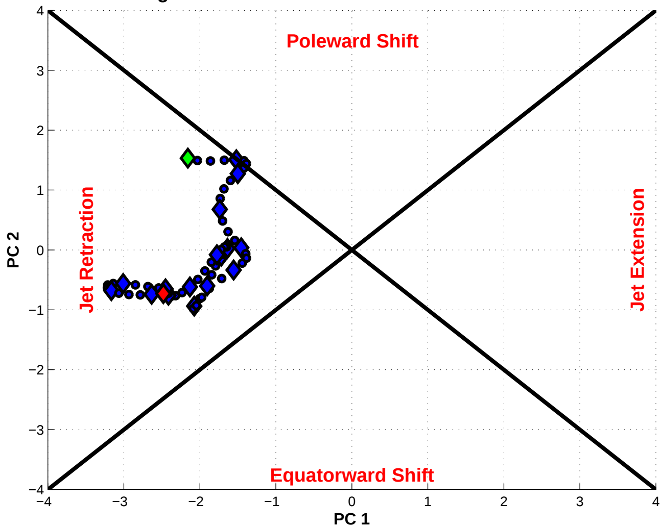
NPJ Phase Diagram valid 0600 UTC 14 Feb 2009 – 1200 UTC 02 Mar 2009
