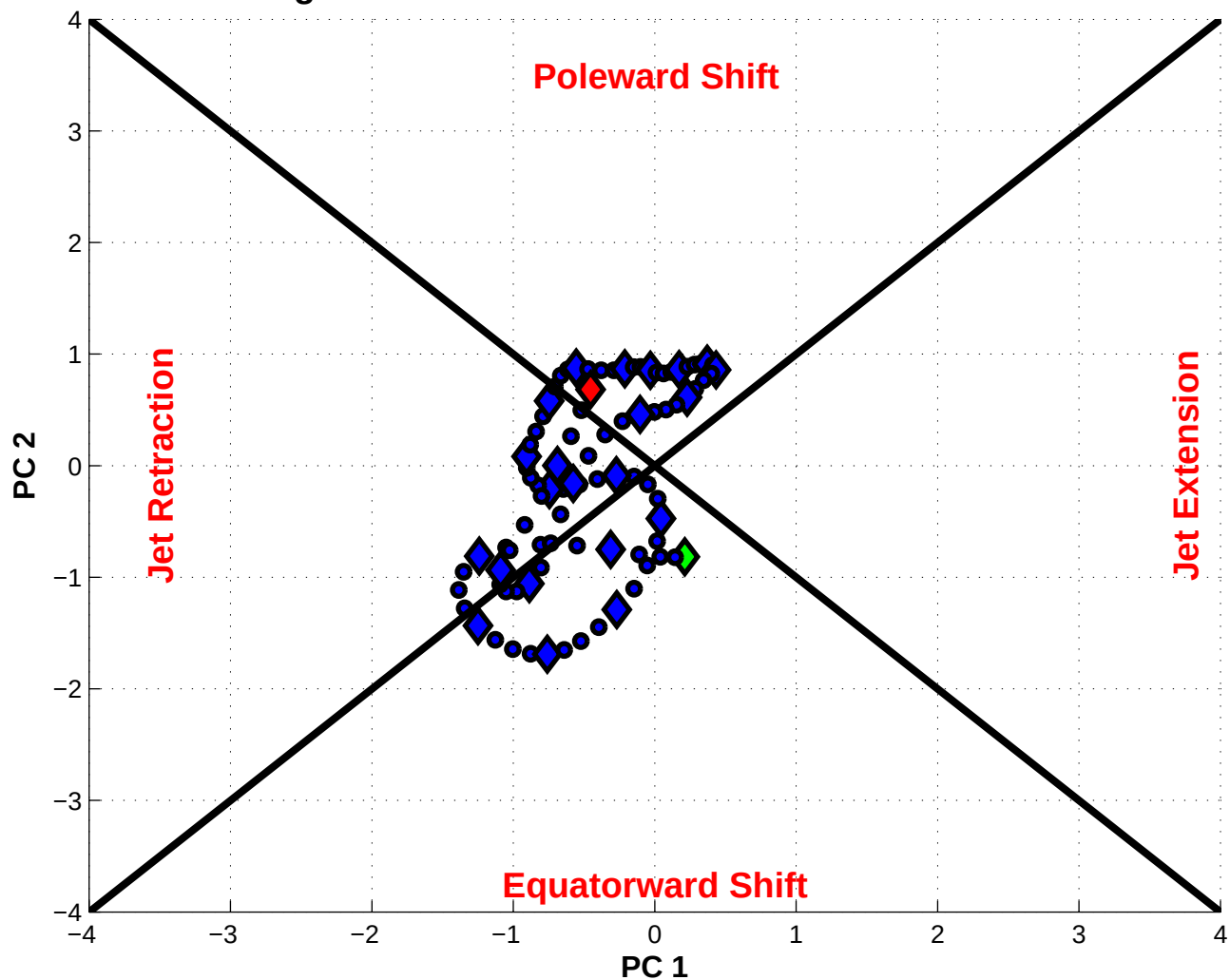
NPJ Phase Diagram valid 1200 UTC 14 Jan 1984 – 0600 UTC 06 Feb 1984
