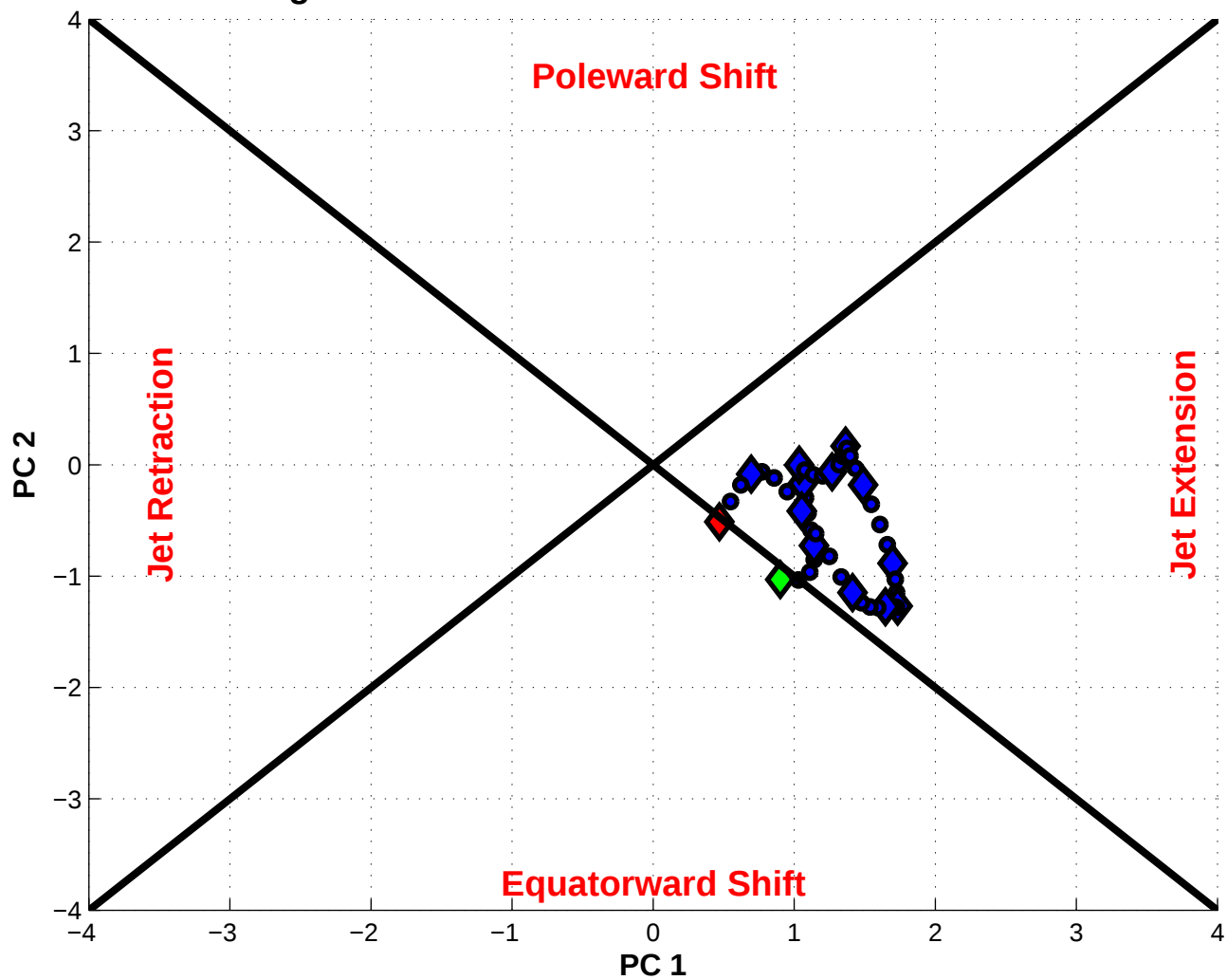
NPJ Phase Diagram valid 1200 UTC 14 Nov 2005 – 0600 UTC 27 Nov 2005
