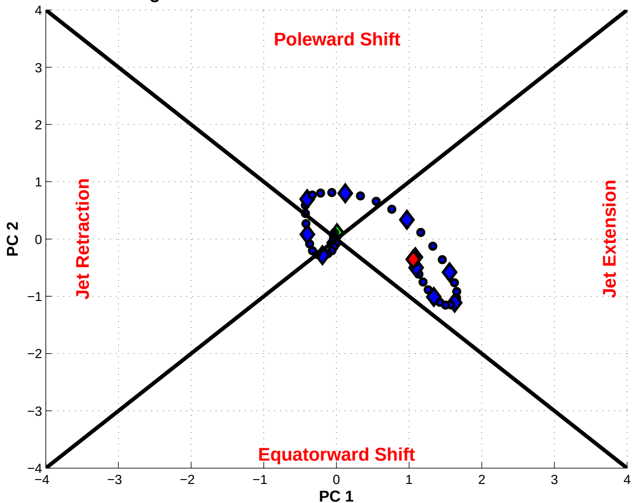
NPJ Phase Diagram valid 1200 UTC 19 Dec 1993 – 0000 UTC 31 Dec 1994
