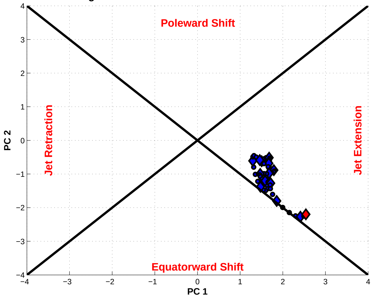
NPJ Phase Diagram valid 1200 UTC 20 Feb 1986 – 0000 UTC 06 Mar 1986
