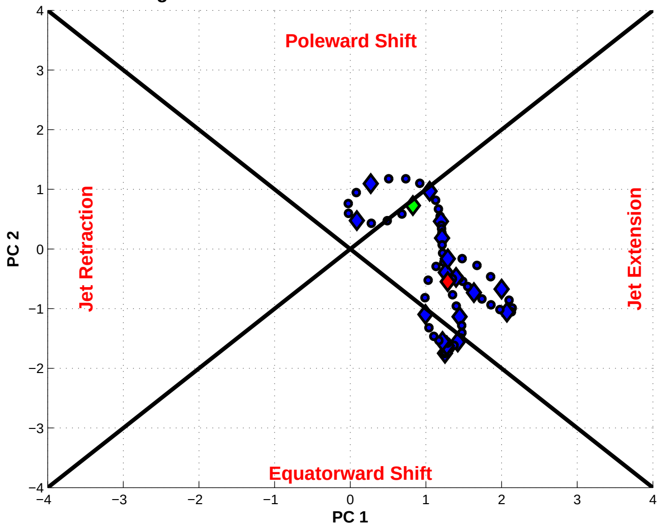
NPJ Phase Diagram valid 1800 UTC 21 Dec 2001 – 0600 UTC 08 Jan 2002
