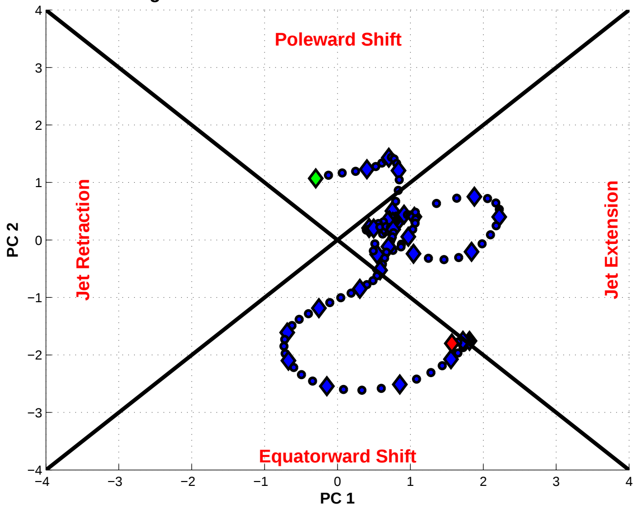
NPJ Phase Diagram valid 0000 UTC 21 Nov 1989 – 1200 UTC 22 Dec 1989
