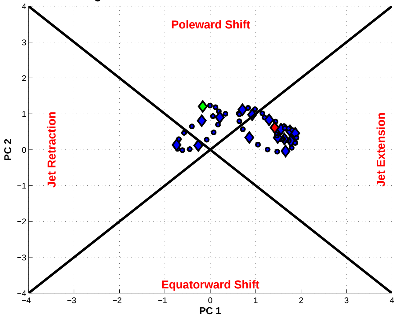
NPJ Phase Diagram valid 1200 UTC 22 Jan 1987 – 1800 UTC 06 Feb 1987
