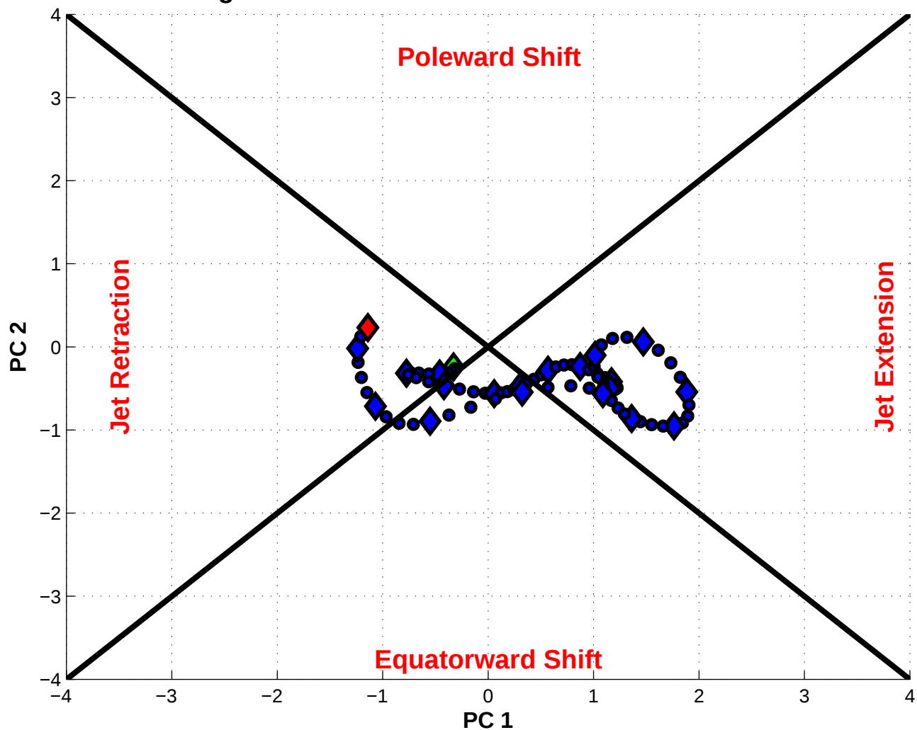
NPJ Phase Diagram valid 1200 UTC 23 Feb 2005 – 0000 UTC 15 Mar 2005
