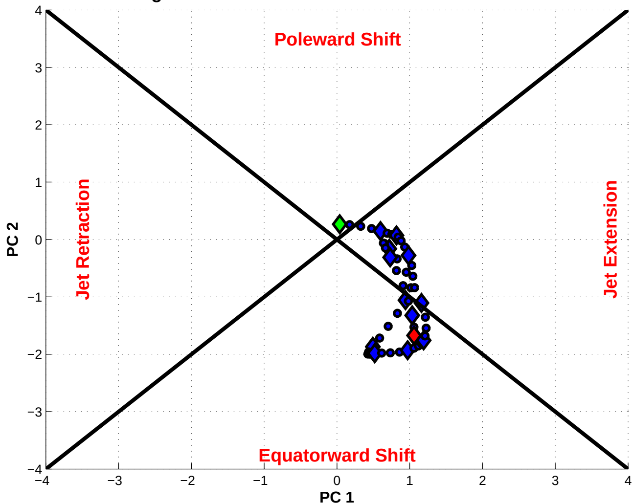
NPJ Phase Diagram valid 0000 UTC 24 Jan 2007 – 1200 UTC 05 Feb 2007
