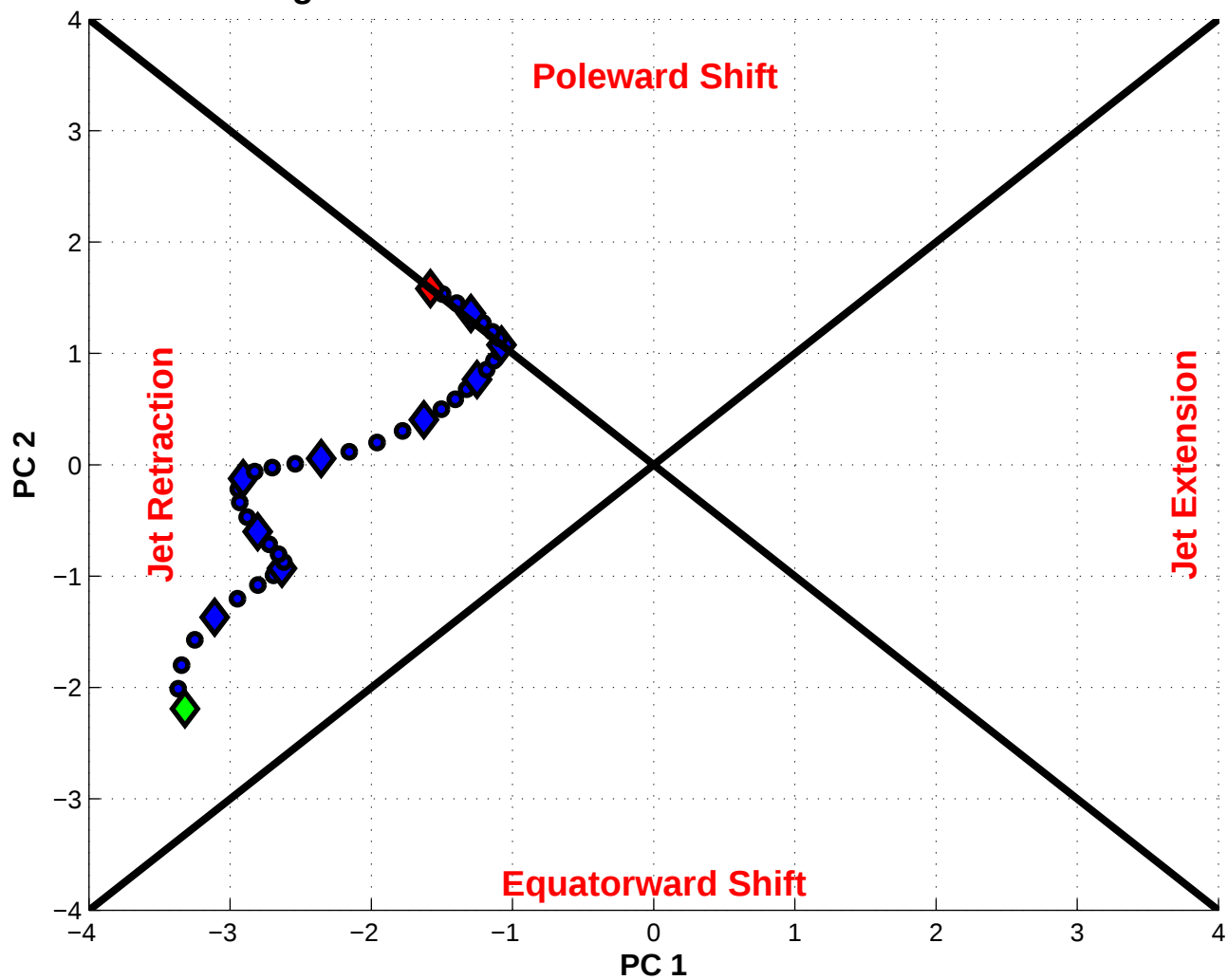
NPJ Phase Diagram valid 1800 UTC 26 Feb 2006 – 1200 UTC 08 Mar 2006
