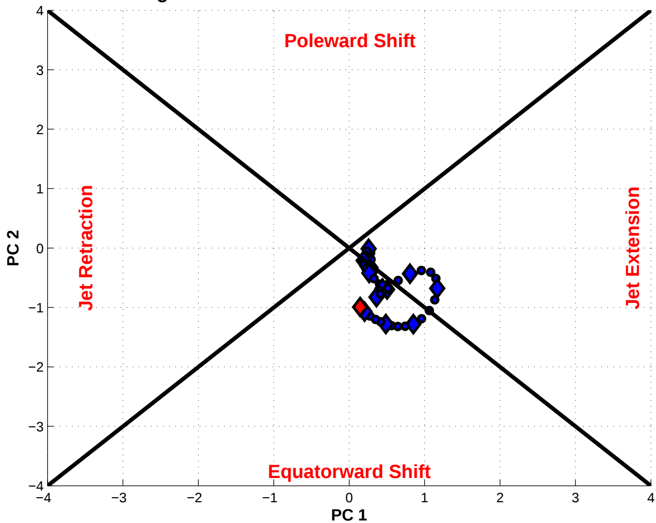
NPJ Phase Diagram valid 1200 UTC 27 Jan 1993 – 1800 UTC 07 Feb 1993
