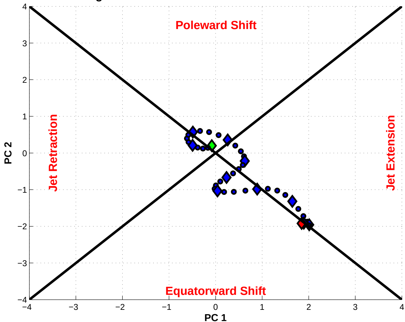
NPJ Phase Diagram valid 0000 UTC 28 Nov 2009 – 0600 UTC 08 Dec 2009
