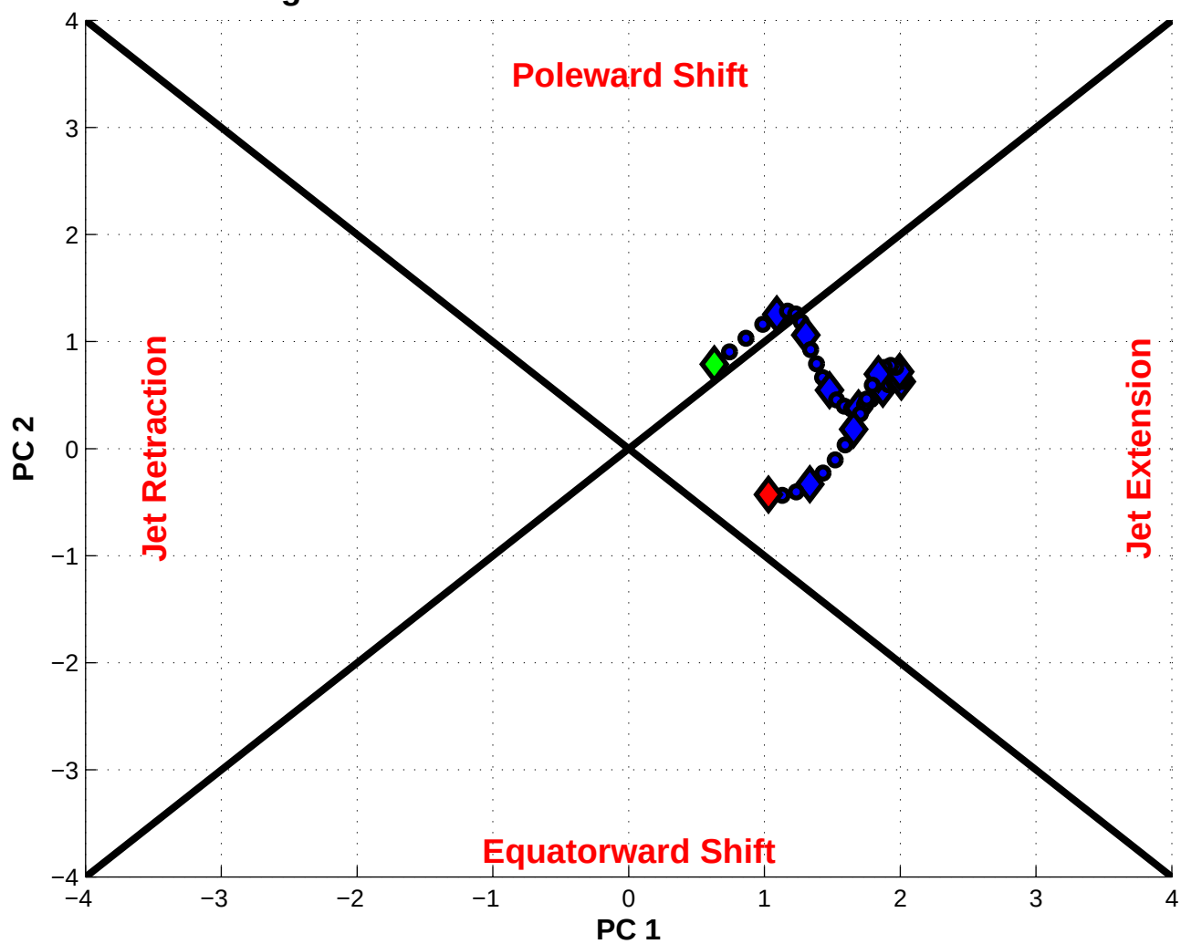
NPJ Phase Diagram valid 0600 UTC 29 Feb 2008 – 0000 UTC 11 Mar 2008
