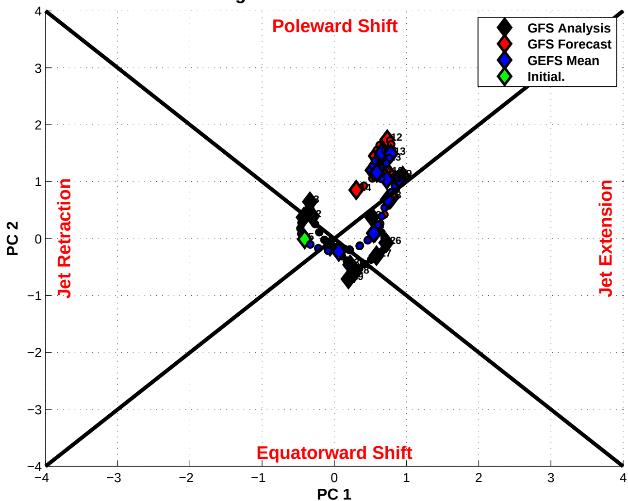
NPJ Phase Diagram initialized 0000 UTC 05 Oct 2016
