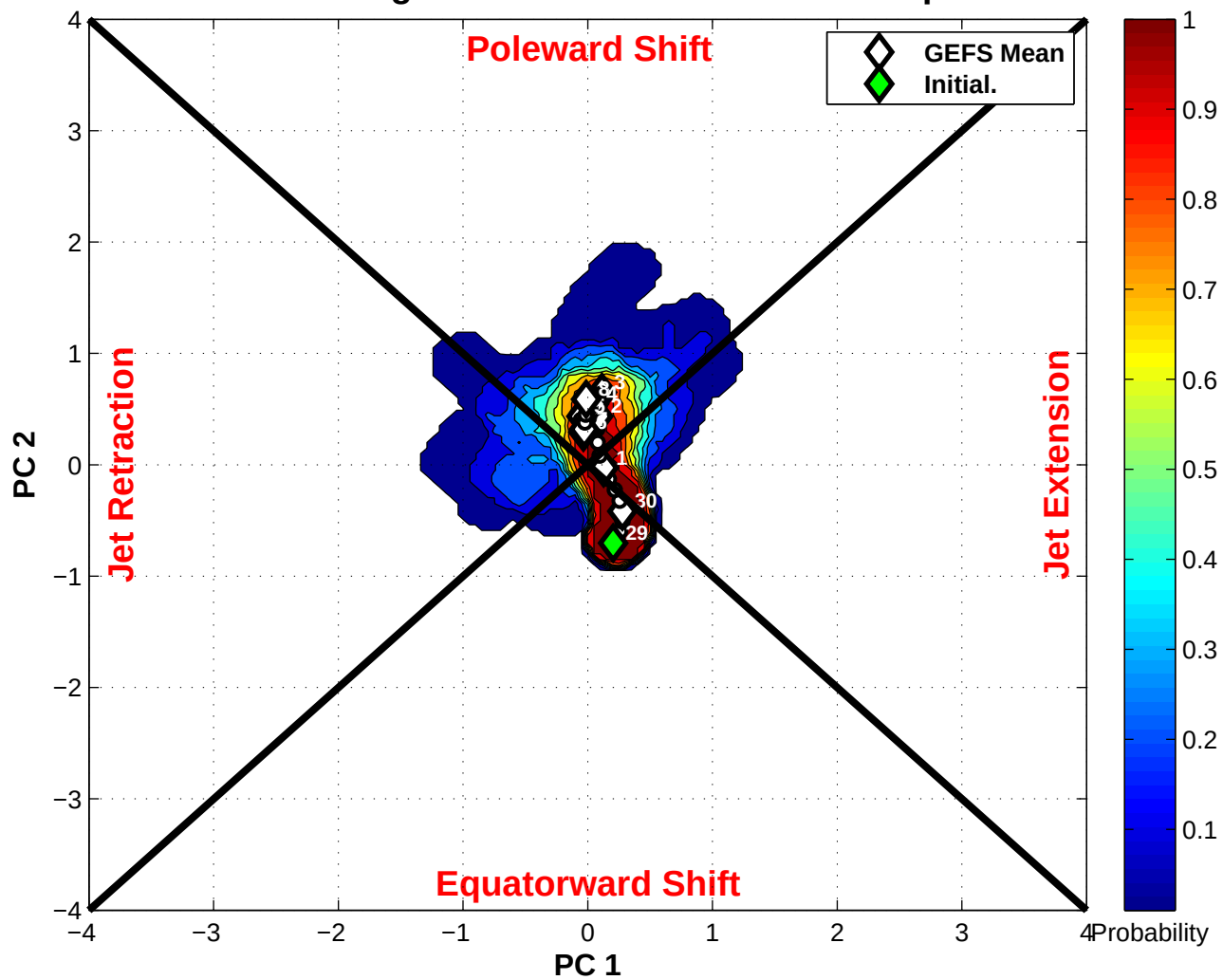
NPJ Phase Diagram initialized 0000 UTC 29 Sep 2016
