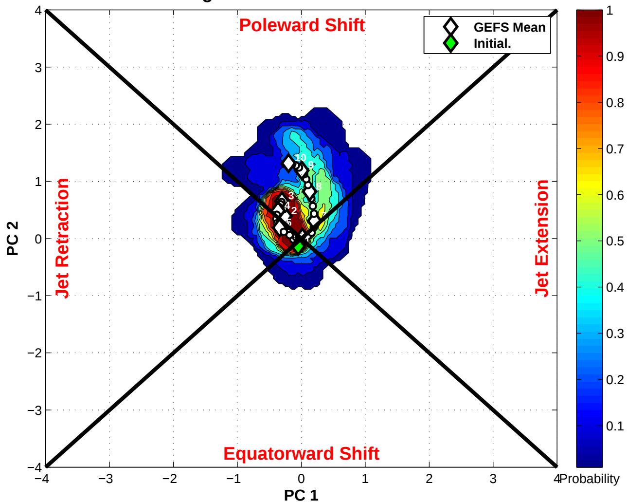
NPJ Phase Diagram initialized 0000 UTC 01 Oct 2016
