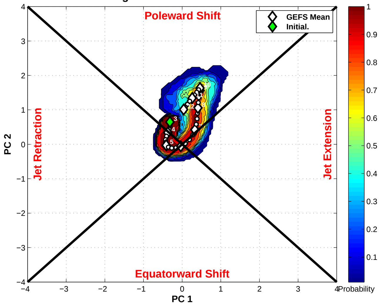
NPJ Phase Diagram initialized 0000 UTC 03 Oct 2016
