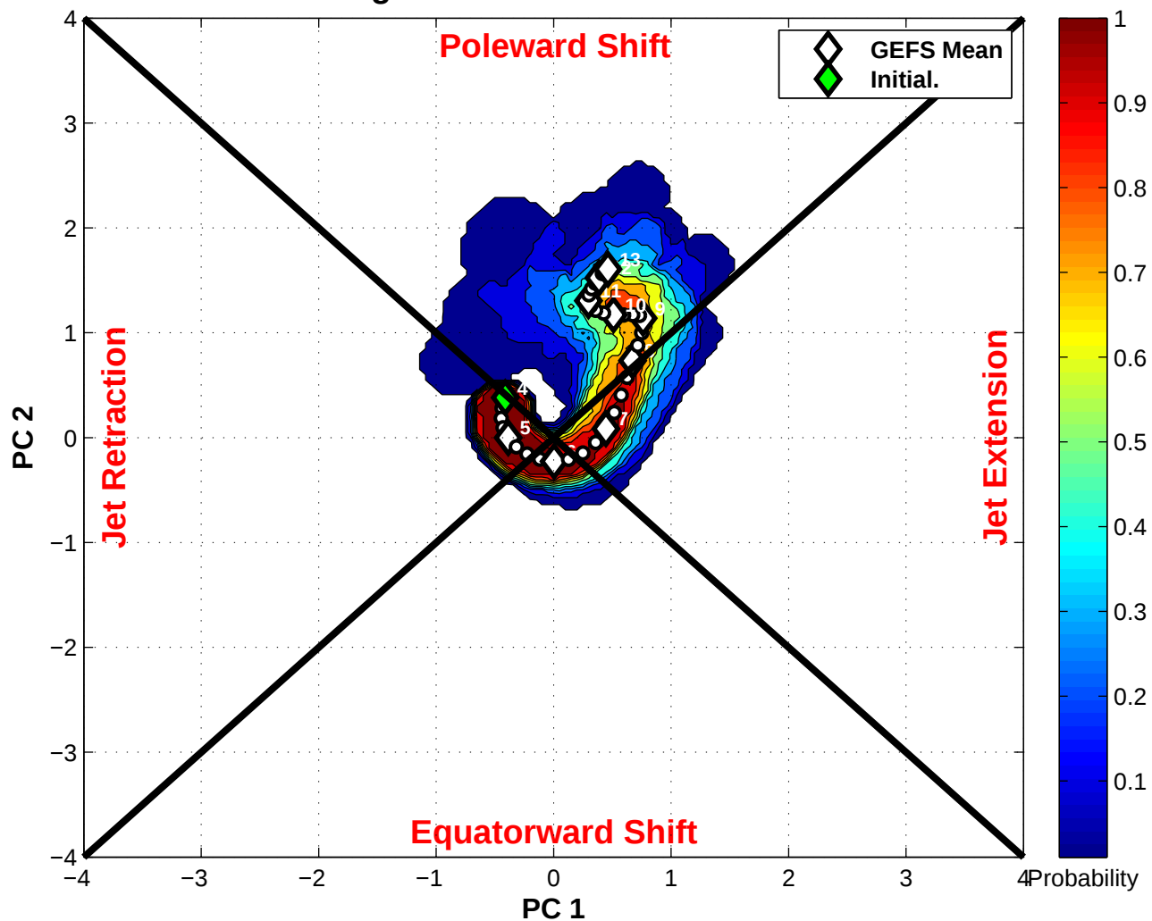
NPJ Phase Diagram initialized 0000 UTC 04 Oct 2016
