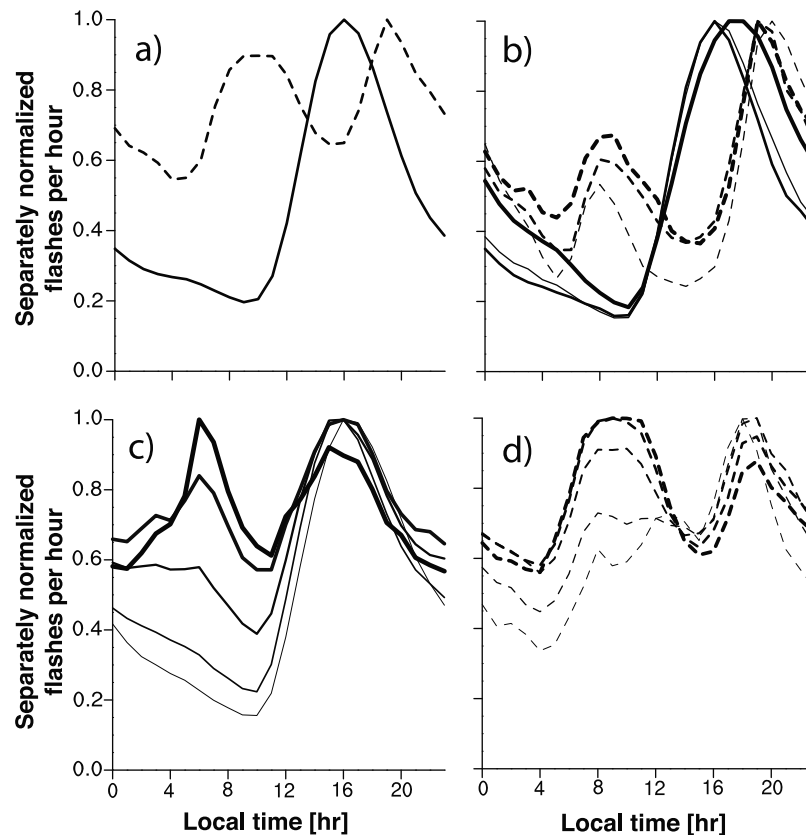
Figure 5. Diurnal cycle as captured by the NLDN (solid lines) and the WWLLN (dashed lines), for (a) the domain of the study (25°N–45°N and 125°W–75°W) and (b) for a domain including only continent (32°N–45°N and 115°W–82°W). (b) The thin lines correspond to the year 2006–2007, the medium lines correspond to 2007–2008, and the thick lines correspond to 2008–2009. (c) Contains the diurnal cycle as captured by the NLDN in bins of 30 kA, for negative flashes in the continent-only domain. The thinnest line corresponds to the weakest flashes (up to -30 kA), and the thickest line corresponds to the strongest flashes considered ( -120 to -150 kA). (d) Same as Figure 5c but for the WWLLN. Each (1 h) time bin and network is normalized independently to facilitate comparison.
