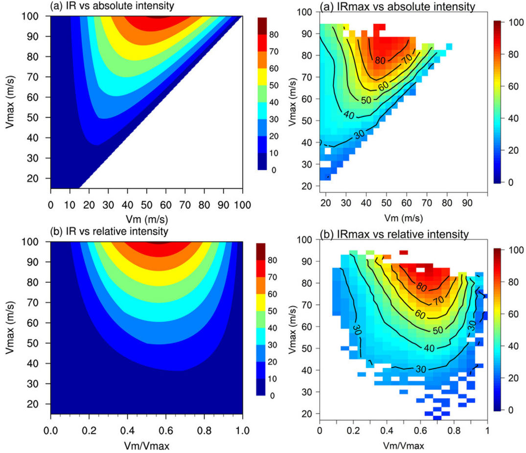
Fig. 9. Left column: Distribution of intensification rates ( \text{m s}^{-1} \text{ day}^{-1} ) as a function of (top) TC intensity ( V_m ) and MPI ( V_{max} ), and (bottom) relative TC intensity ( V_m/V_{max} ) and V_{max} calculated using Equation (3). Right column: Distribution of the 99th percentile of intensification rates as a function of (top) V_m and V_{max} , and (bottom) V_m/V_{max} and V_{max} using the 6-hourly maximum 10-m sustained wind speed based on the best-track data of TCs in SHIPS (Knaff et al. 2005). Adapted from Figs. 2 and 5 in Wang et al. (2021b).
