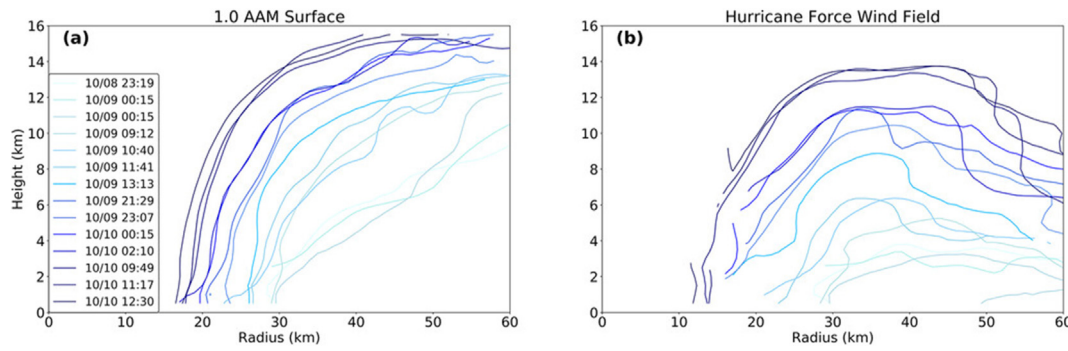
Fig. 7. (a) Progression of the azimuthally-averaged 10^6 \text{ m}^2 \text{ s}^{-1} absolute angular momentum (AAM) contour, and (b) hurricane-force wind contour ( 33 \text{ m s}^{-1} ) during 14 aircraft passes in Hurricane Michael (2018). Adapted from Fig. 3 in DesRosiers et al. (2022).
