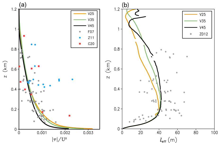
Fig. 3. Vertical profiles of nondimensionalized vertical turbulent momentum flux \tau ( \text{m}^2 \text{ s}^{-2} ) from three LES experiments where the surface wind speed is 25 \text{ m s}^{-1} (V25, orange), 35 \text{ m s}^{-1} (V35, green), and 45 \text{ m s}^{-1} (V45, black). Gray and blue dots denote previous aircraft observations, and red dots denote the sUAS data from Cione et al. (2020). (b) Vertical profiles of the effective mixing length l_{eff} from the three LES experiments. Adapted from Figs. 7 and 11 in Chen et al. (2021a).
