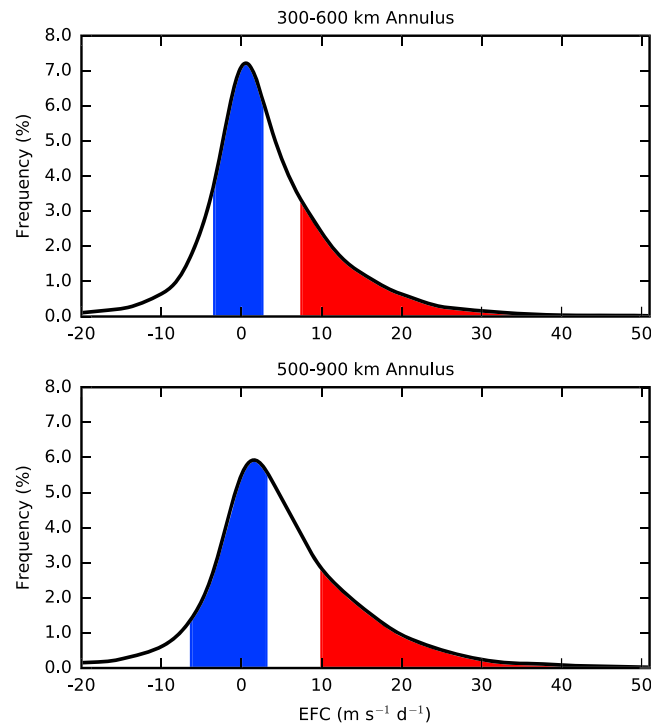
Figure 1. Distributions of 200 hPa EFC in the (top) 300–600 km annulus and (bottom) 500–900 km annulus for all eligible 6 h time periods. Red shading indicates \text{EFC} \geq 75\text{th percentile} . Blue shading indicates EFC within \pm 20 percentiles of \text{EFC} = 0 \text{ m s}^{-1} \text{ d}^{-1} .
