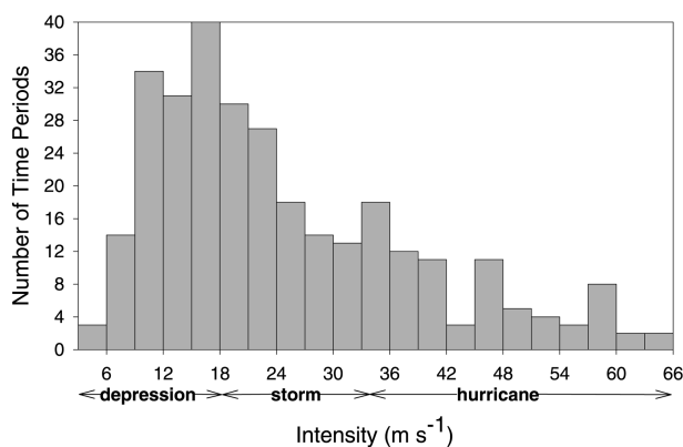
FIG. A2. Distribution of average intensity (defined by the maximum surface wind speed in \text{m s}^{-1} ) for all 303 12-h time periods. The conventional classes of tropical cyclone strength are noted for reference.
