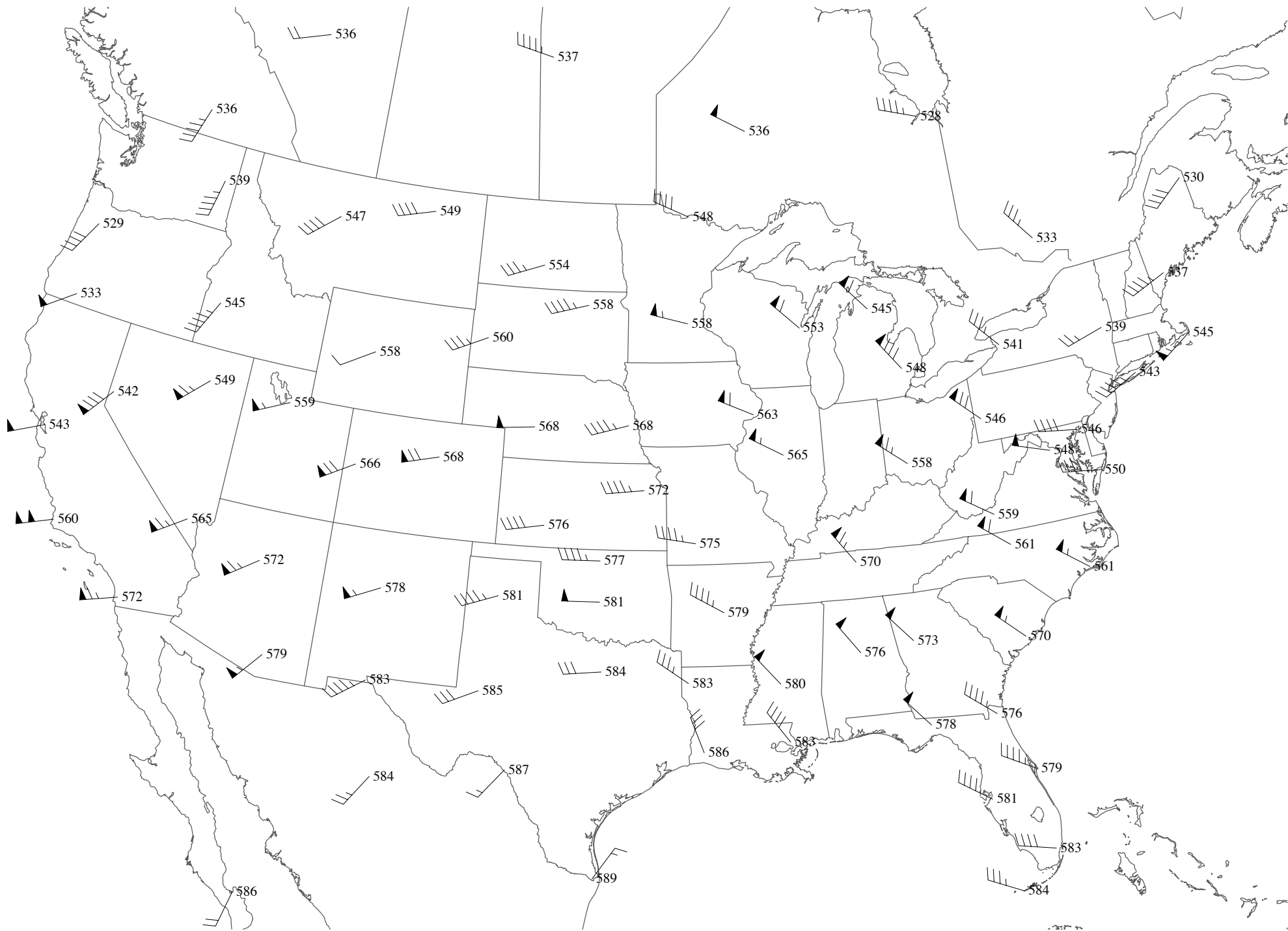
160218/1200 500-mb Height and Wind – Contour every 6 dam
