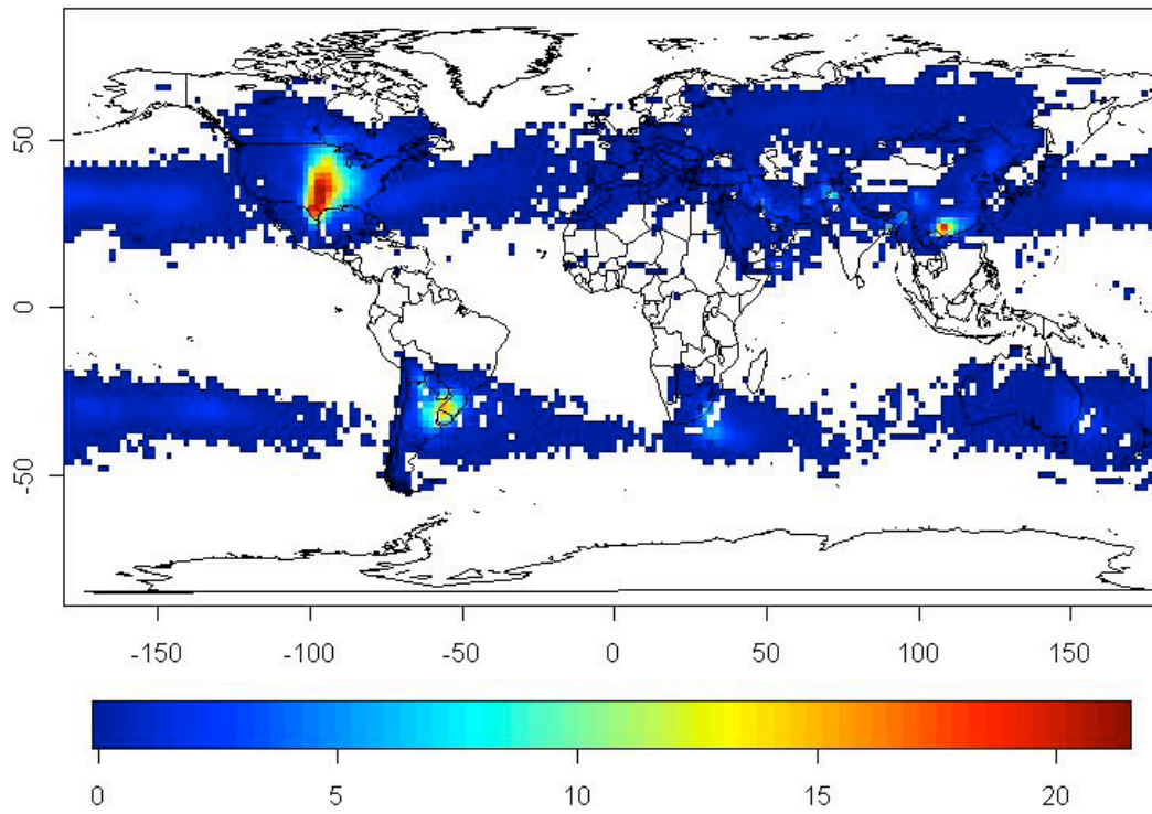
Annual Mean Tornadic Environment Periods (1970-1999)
