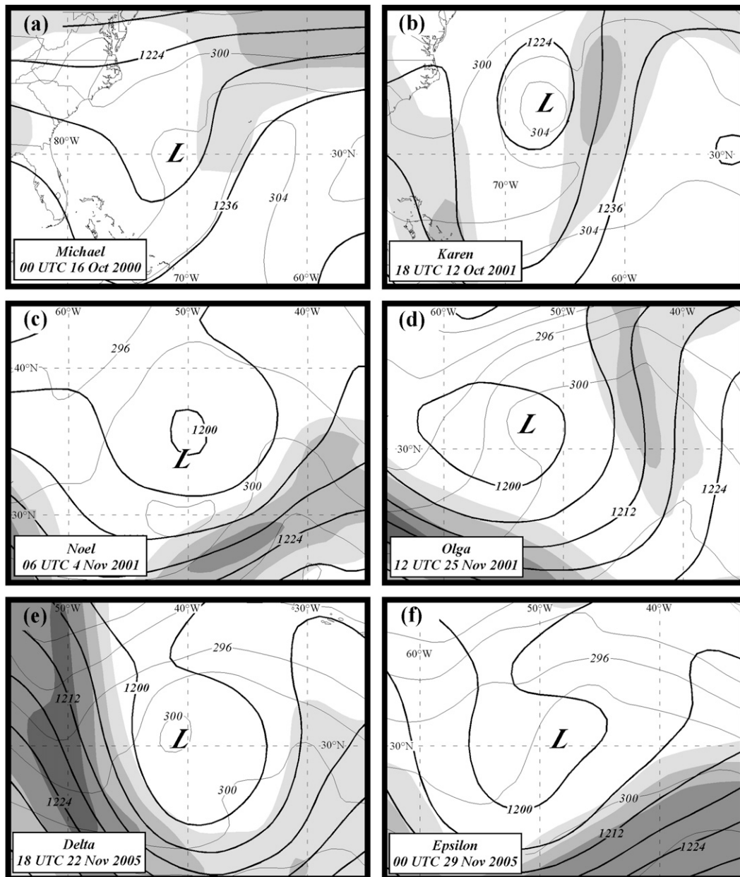
FIG. 11. As in Fig. 2, but for (a) 0000 UTC 16 Oct 2000 (Michael), (b) 1800 UTC 12 Oct 2001 (Karen), (c) 0600 UTC 4 Nov 2001 (Noel), (d) 1200 UTC 25 Nov 2001 (Olga), (e) 1800 UTC 22 Nov 2005 (Delta), and (f) 0000 UTC 29 Nov 2005 (Epsilon).
