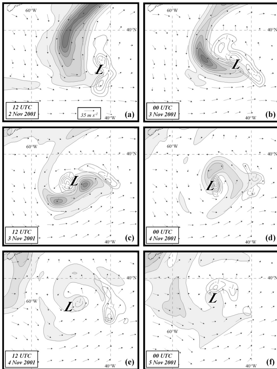
FIG. 7. FNL analyses of 325–335-K PV (PVU, filled), 330-K winds (arrows), and 330-K diabatic PV tendency (gray lines) for (a) 1200 UTC 2 Nov 2001, (b) 0000 UTC 3 Nov 2001, (c) 1200 UTC 3 Nov 2001, (d) 0000 UTC 4 Nov 2001, (e) 1200 UTC 4 Nov 2001, and (f) 0000 UTC 5 Nov 2001. PV contoured and shaded every 1 PVU beginning at 1 PVU. Diabatic PV tendency labeled in PVU day -1 and contoured every 0.5 PVU day -1 beginning at -0.5 PVU day -1 . The "L" in (a)–(f) represents position of the SLP minimum.
