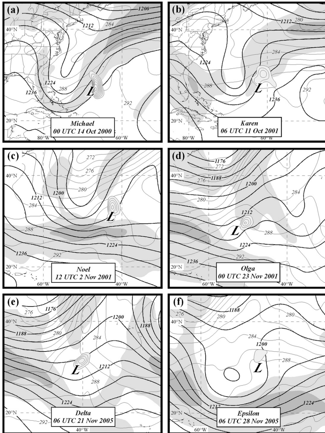
FIG. 2. FNL analyses of 200-hPa geopotential height, 900-hPa temperature, PVA by the thermal wind, and 200-hPa wind speed for (a) 0000 UTC 14 Oct 2000 (Michael), (b) 0600 UTC 11 Oct 2001 (Karen), (c) 1200 UTC 2 Nov 2001 (Noel), (d) 0000 UTC 23 Nov 2001 (Olga), (e) 0600 UTC 21 Nov 2005 (Delta), and (f) 0600 UTC 28 Nov 2005 (Epsilon). Thick black lines are geopotential height labeled in dam and contoured every 6 dam. Thin gray lines are 900-hPa temperature labeled in K and contoured every 2 K. Thin black lines (with shading) are regions of positive advection of 700-hPa geostrophic vorticity by the 500–900-hPa thermal wind, labeled in 10^{-9} \text{ m kg}^{-1} and contoured every 2 \times 10^{-9} \text{ m kg}^{-1} starting at 2 \times 10^{-9} \text{ m kg}^{-1} . Shaded regions are 200-hPa wind speeds shaded every 20 \text{ m s}^{-1} starting at 25 \text{ m s}^{-1} . The “L” in (a)–(f) represents the position of the SLP minimum.
