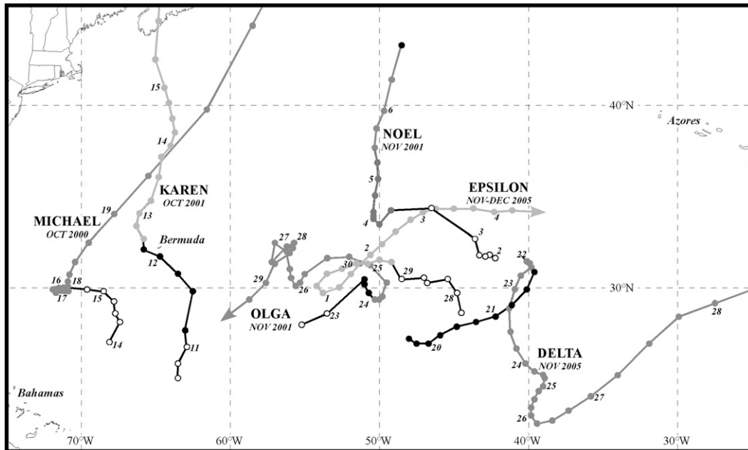
FIG. 1. Cyclone tracks of each of the six tropical transition cases. Closed dots represent cyclone positions taken from HURDAT with open dots indicating supplemental cyclone positions taken from FNL analysis. Black lines/dots indicate positions at which the cyclone was considered nontropical (either extratropical or subtropical) and gray lines/dots indicates position at which the cyclone was considered tropical (note that different shades of gray have no significance except to demarcate different tracks). Number next to a dot indicates the 0000 UTC position for that date. Cyclone tracks lasting 5 days after tropical transition are truncated and end in an arrow.
