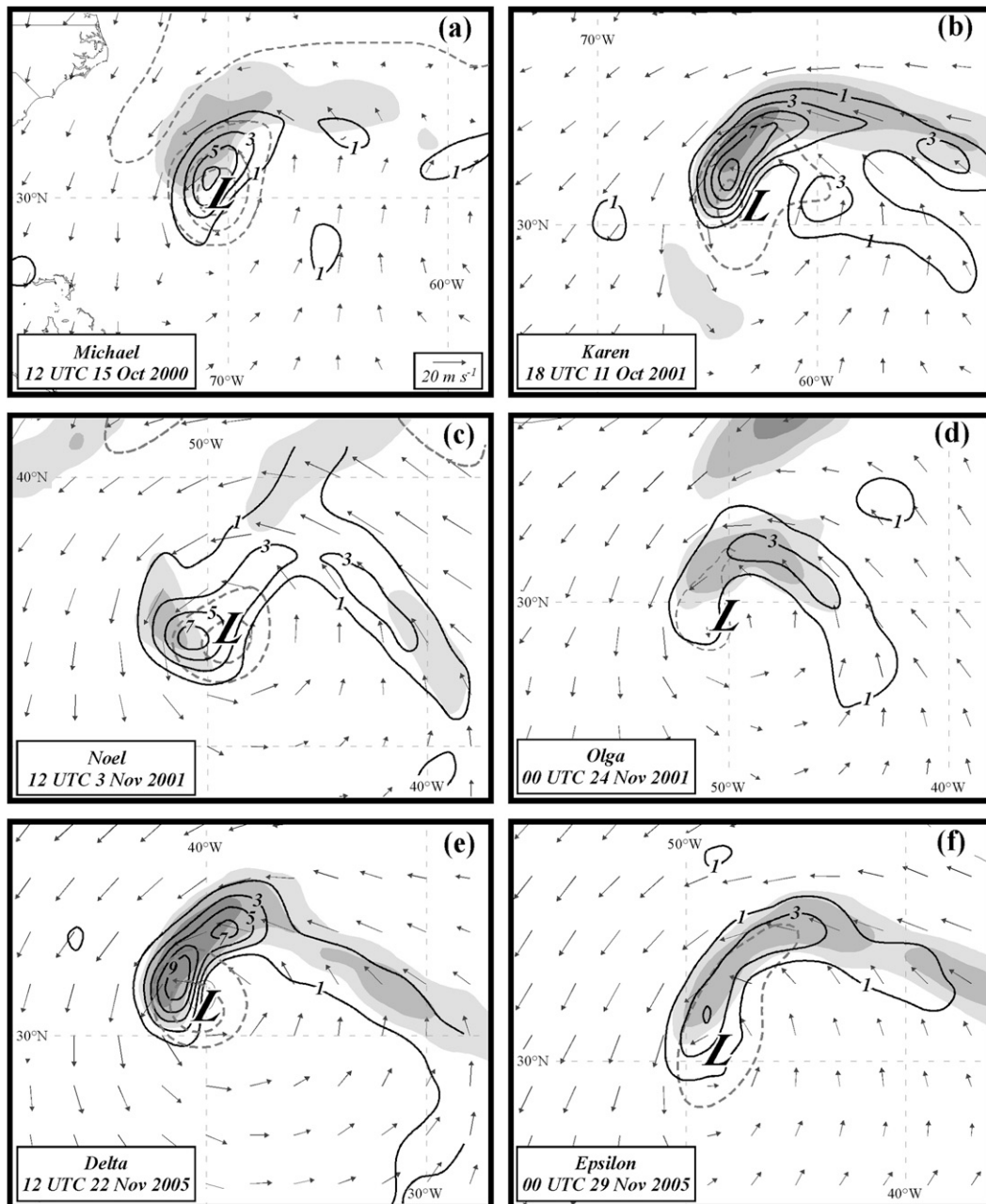
FIG. 4. As in Fig. 3, but FNL analyses of 900-hPa frontogenesis (shaded), 850–950-hPa PV (dashed gray lines), and 900-hPa diabatic PV tendency. Frontogenesis shaded as in Fig. 3 and PV labeled and contoured, though with dashed lines, as in Fig. 3. Diabatic PV tendency is labeled in \text{PVU day}^{-1} and contoured every 2 \text{ PVU day}^{-1} beginning at 1 \text{ PVU day}^{-1} .
