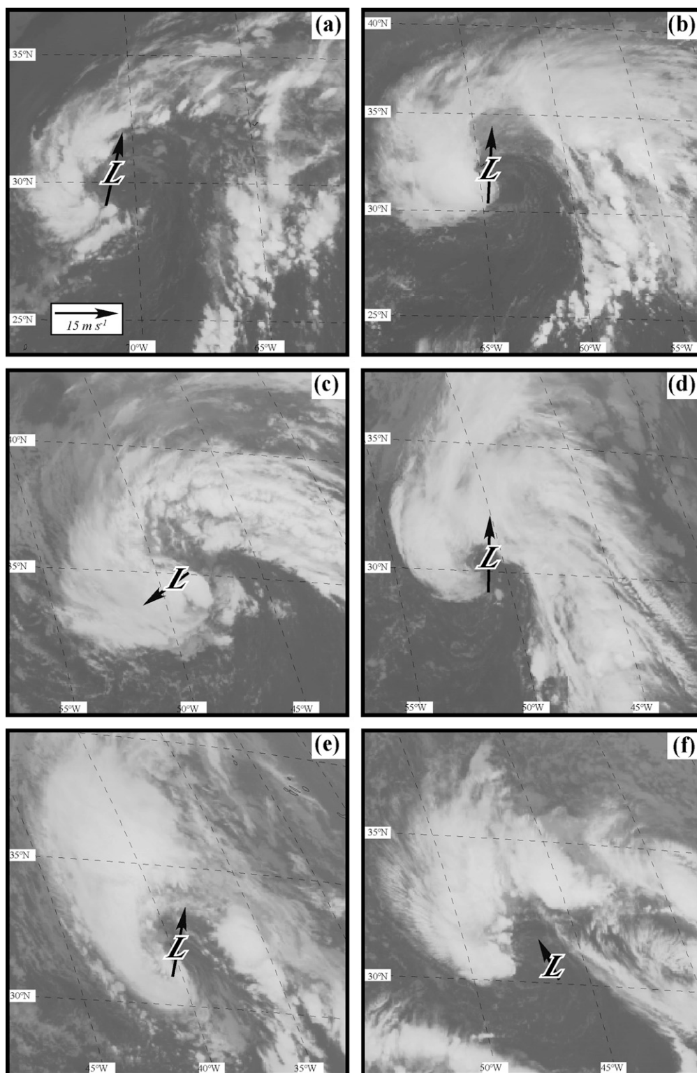
FIG. 9. Infrared satellite images from (a) 1115 UTC 15 Oct 2000 (Michael), (b) 2215 UTC 11 Oct 2001 (Karen), (c) 0915 UTC 3 Nov 2001 (Noel), (d) 0815 UTC 23 Nov 2001 (Olga), (e) 0415 UTC 22 Nov 2005 (Delta), and (f) 1115 UTC 28 Nov 2005 (Epsilon). Thick black arrow in (a)–(f) indicates the direction and magnitude of the 200–900-hPa vertical shear over the cyclone center determined as in Table 2.
