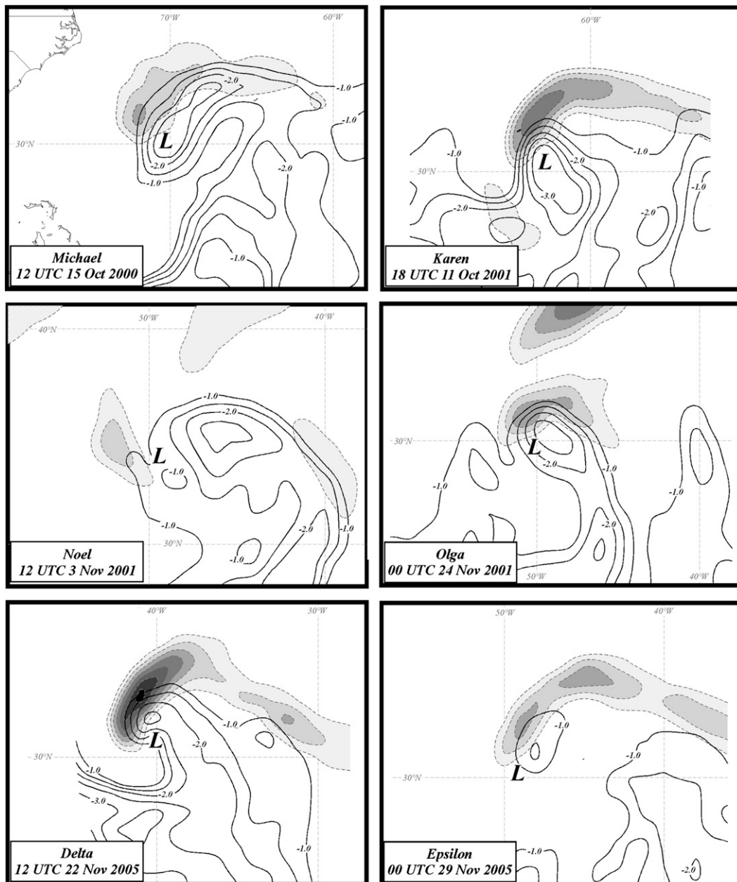
FIG. 12. FNL analyses of 900-hPa positive frontogenesis (dashed lines with shading) and negative 900–500-hPa \theta_e lapse rate (solid lines) for (a) 1200 UTC 15 Oct 2000 (Michael), (b) 1800 UTC 11 Oct 2001 (Karen), (c) 1200 UTC 3 Nov 2001 (Noel), (d) 0000 UTC 24 Nov 2001 (Olga), (e) 1200 UTC 22 Nov 2005 (Delta), and (f) 0000 UTC 29 Nov 2005 (Epsilon). Frontogenesis labeled, contoured, and shaded as in Fig. 3. The 500–900-hPa \theta_e lapse rate is labeled in \text{K km}^{-1} and contoured every -0.5 \text{ K km}^{-1} beginning at -0.5 \text{ K km}^{-1} . The “L” in (a)–(f) represents the position on the SLP minimum.
