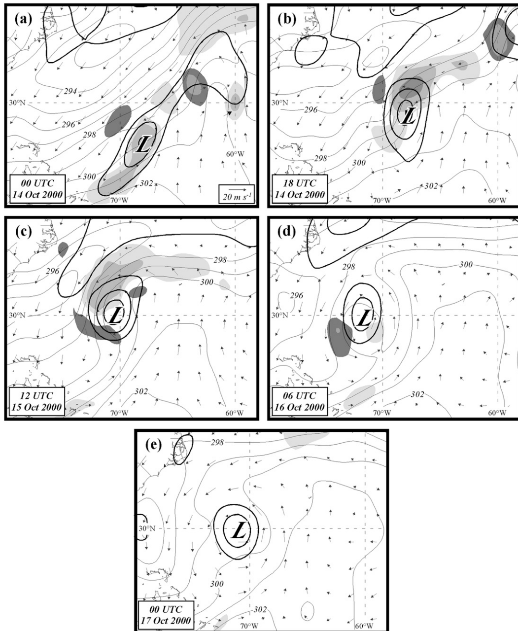
FIG. 5. As in Fig. 3, but for (a) 0000 UTC 14 Oct 2000, (b) 1800 UTC 14 Oct 2000, (c) 1200 UTC 15 Oct 2000, (d) 0600 UTC 16 Oct 2000, and (e) 0000 UTC 17 Oct 2000.
