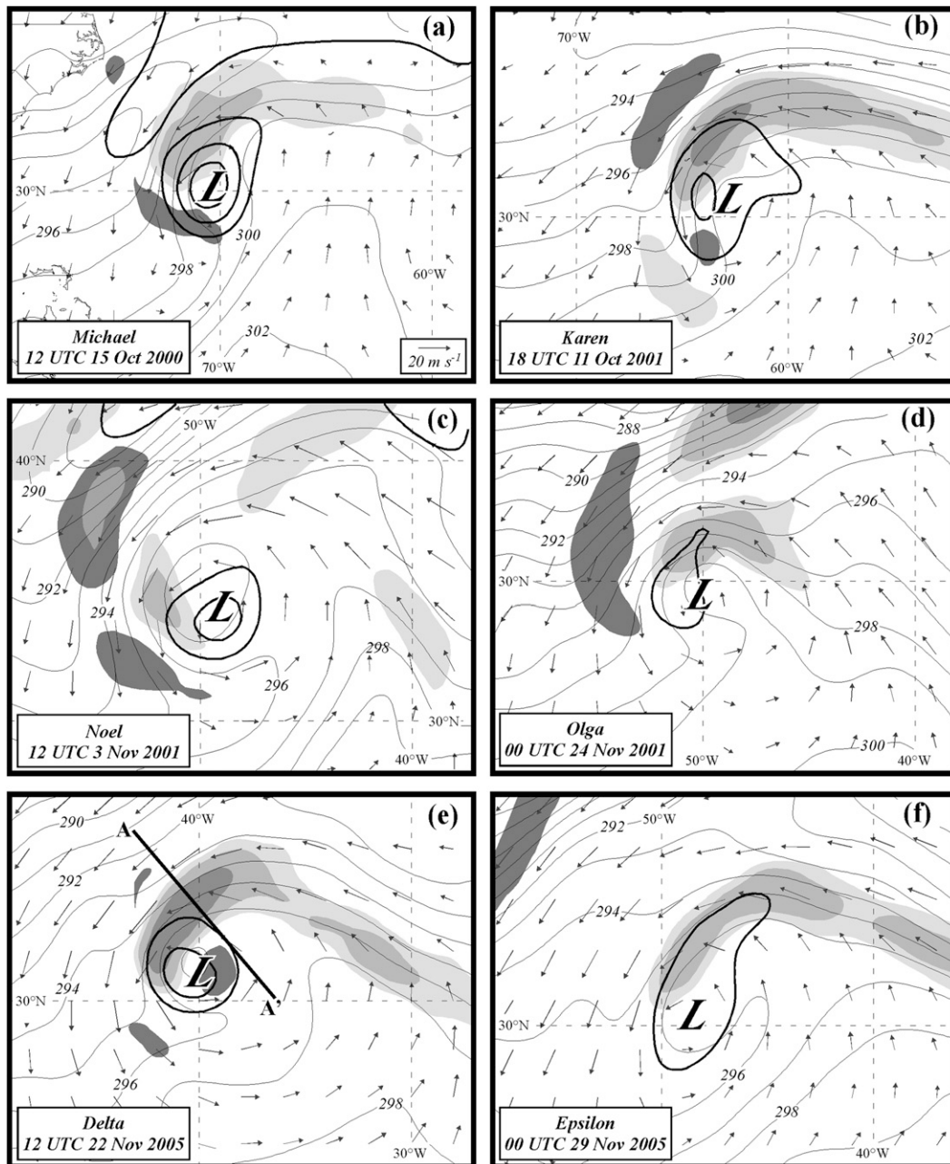
FIG. 3. FNL analyses of 850–950-hPa PV (thick black lines), 900-hPa potential temperature (thin gray lines), and 900-hPa frontogenesis (shaded) for (a) 1200 UTC 15 Oct 2000 (Michael), (b) 1800 UTC 11 Oct 2001 (Karen), (c) 1200 UTC 3 Nov 2001 (Noel), (d) 0000 UTC 24 Nov 2001 (Olga), (e) 1200 UTC 22 Nov 2005 (Delta), and (f) 0000 UTC 29 Nov 2005 (Epsilon). Temperature is labeled in K and contoured every 2 K. PV is labeled in PVU ( 1 \text{ PVU} \equiv 10^{-6} \text{ m}^2 \text{ K kg}^{-1} \text{ s}^{-1} ) and contoured every 0.25 PVU beginning at 0.5 PVU. Frontogenesis is contoured in frontogenesis units [ \text{FGU} = \text{K} (100 \text{ km})^{-1} (3 \text{ h})^{-1} ] and is shaded every 0.2 FGU with light (dark) shading indicating positive (negative) frontogenesis. The “L” in (a)–(f) represents position of the SLP minimum.
