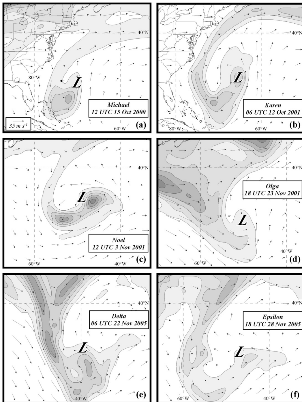
FIG. 8. FNL analyses of (a) 335–345-K PV (PVU, filled) and 340-K winds (arrows) for 1200 UTC 15 Oct 2000 (Michael), (b) 335–345-K PV and 340-K winds for 0600 UTC 12 Oct 2001 (Karen), (c) 325–335-K PV and 330-K winds for 1200 UTC 3 Nov 2001 (Noel), (d) 330–340-K PV and 335-K winds for 1800 UTC 23 Nov 2001 (Olga), (e) 330–340-K PV and 335-K winds for 0600 UTC 22 Nov 2005 (Delta), and (f) 325–335-K PV and 330-K winds for 1800 UTC 28 Nov 2005 (Epsilon). PV contoured and shaded as in Fig. 7. The “L” in (a)–(f) represents position of the SLP minimum.
