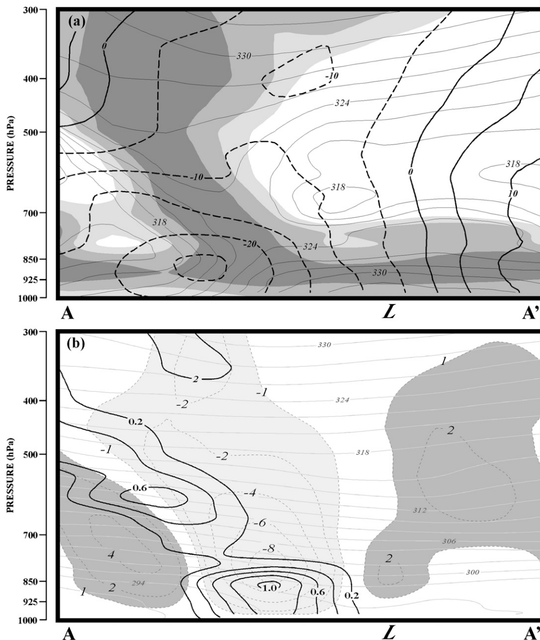
FIG. 10. Cross section, along A–A' in Fig. 3e, from the FNL analysis at 1200 UTC 22 Nov 2005. (a) Thick lines are contours of wind speed normal to the cross section ( \text{m s}^{-1} , values hatched coming out of the page), thin lines are contours of equivalent potential temperature ( \theta_e , K), and shaded areas represent relative humidity. (b) Thin gray lines are isentropes labeled in K and contoured every 2 K. Thick black lines are positive frontogenesis labeled in FGU and contoured every 0.2 FGU beginning at 0.2 FGU. Thin dashed lines are \omega , labeled in \text{dPa s}^{-1} and contoured every -2 ( 2 ) \text{dPa s}^{-1} beginning at -2 ( 2 ) \text{dPa s}^{-1} and also including -1 ( 1 ) \text{dPa s}^{-1} contour, with light (dark) shading indicating region of ascent (descent). The “L” on the cross section represents the position of the SLP minimum.
