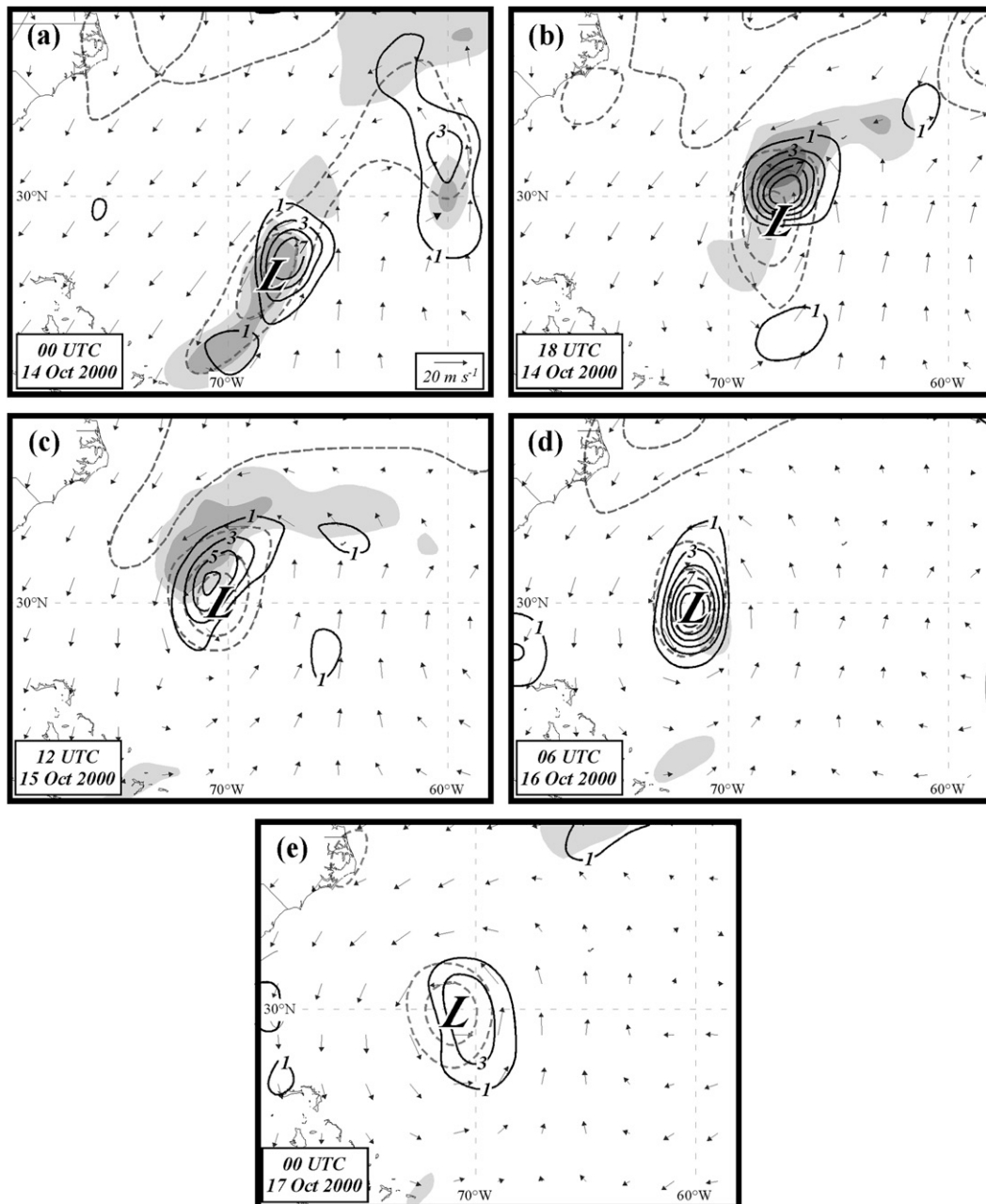
FIG. 6. As in Fig. 4, but for (a) 0000 UTC 14 Oct 2000, (b) 1800 UTC 14 Oct 2000, (c) 1200 UTC 15 Oct 2000, (d) 0600 UTC 16 Oct 2000, and (e) 0000 UTC 17 Oct 2000.
