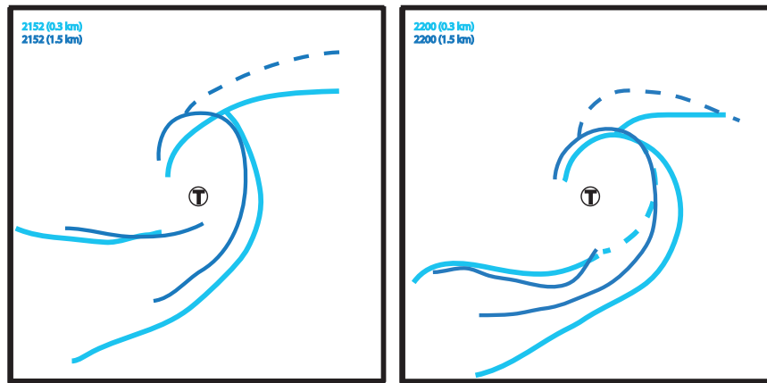
FIG. 10. Locations of the gust fronts at the surface (0.3 km; light blue) and aloft (1.5 km; dark blue) for (left) 2152 and (right) 2200 relative to the tornado (T). The FFG and PRFGF slope backward with height, whereas the SRFGF does not exhibit much slant with height, possibly indicating differences in relative buoyancies across the different boundaries.
