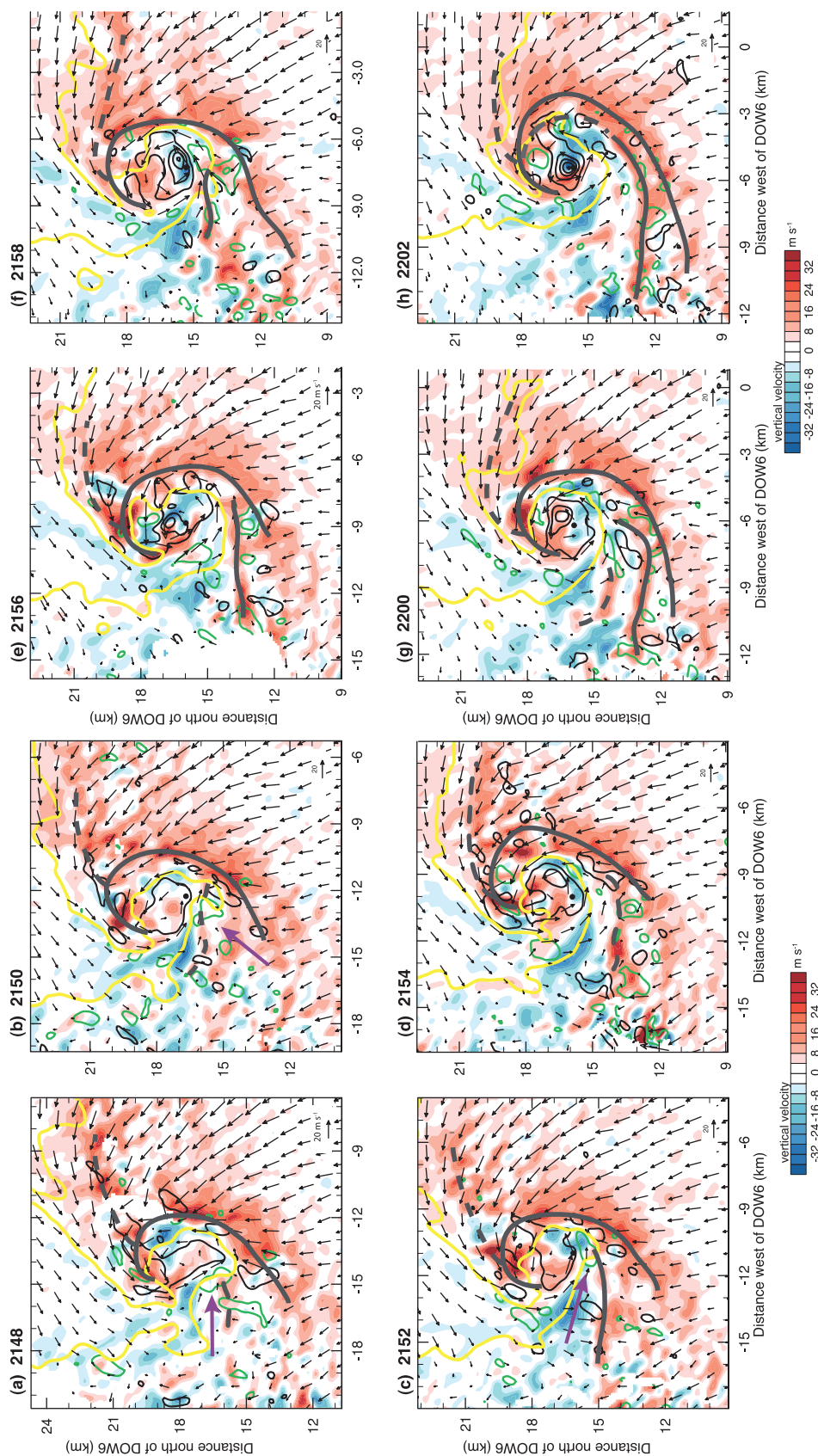
FIG. 9. As in Fig. 7, but at a height of 1.5 km.
