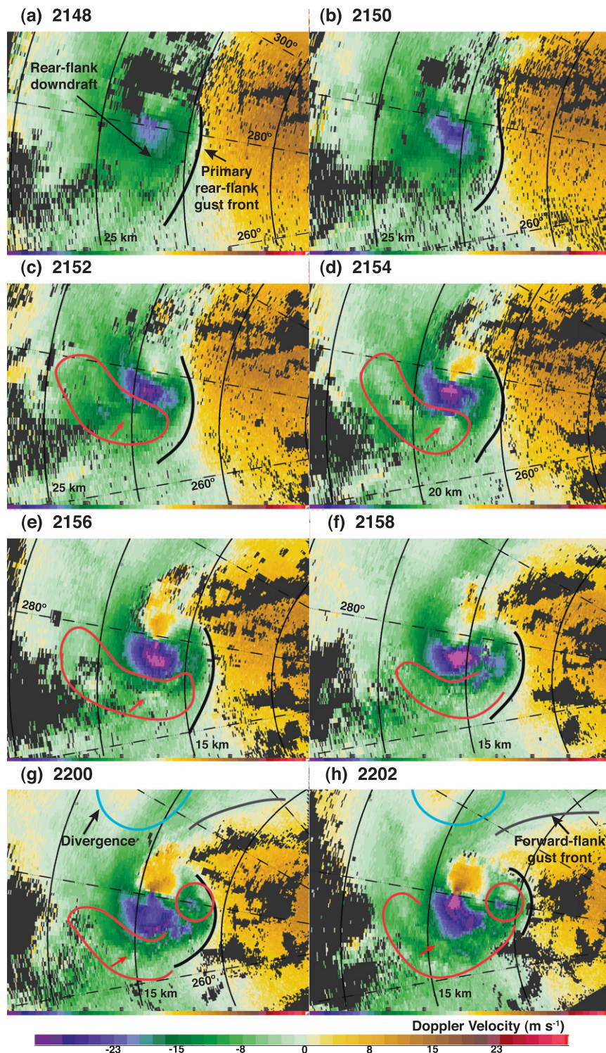
FIG. 5. (a)–(h) Evolution of the Doppler velocity field at 1° elevation as measured by DOW7 (shown every 2 min). By 2152:50 (not shown), the velocity difference across the couplet exceeds 40 \text{ m s}^{-1} , the tornadic threshold established by Alexander and Wurman (2008). Between 2152 and 2202, the RFD wraps east of the tornadic circulation. Red arrows indicate anticyclonic regions, red curves delineate the SRFD and SRFG region, red circles indicate a secondary cyclonic region, and blue curves denote a region of increasing divergence extending north of the displayed panels.
