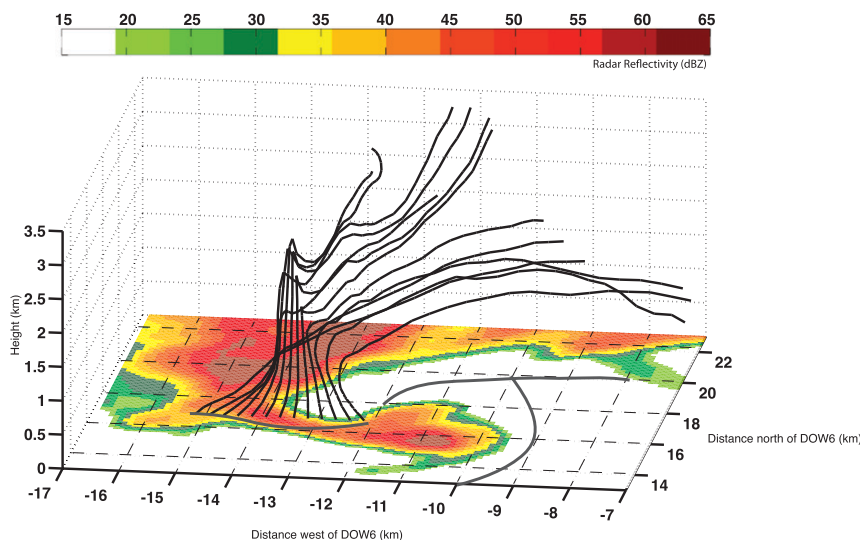
FIG. 15. Backward trajectories starting at 2152 and ending at 2142 for parcels starting just north of the SRFGF. Parcels that composed the SRFD originated a few km aloft. Radar reflectivity is shown at 0.3 km and gray lines denote the locations of the gust fronts. The view is from the south-southeast.
