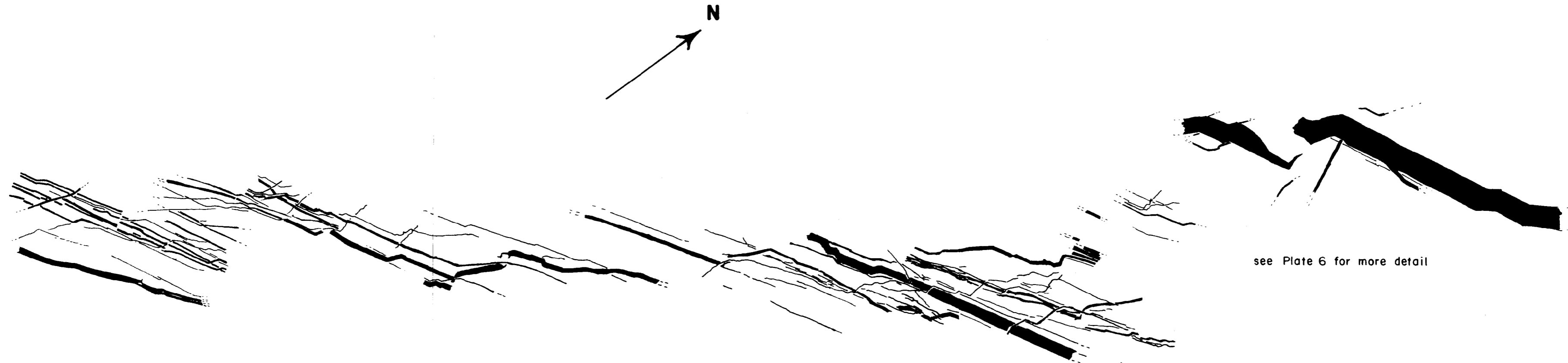
PATTERN OF MESOZOIC DIKE INTRUSION BALD HEAD SOUTH TO POND ROCKS
